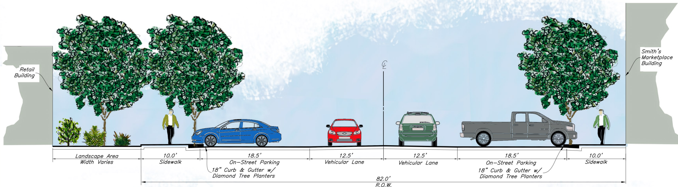
1. Secondary Street Type "A" Cross Section
