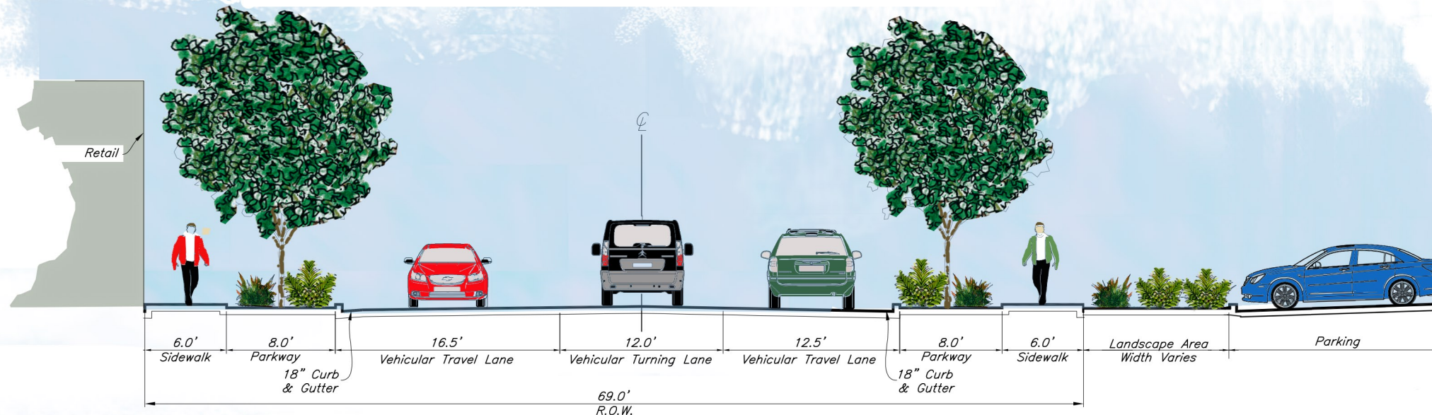
2. Secondary Street Type "B1" Cross Section
