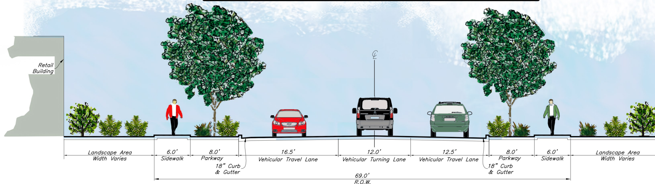
3. Secondary Street Type "B2" Cross Section
