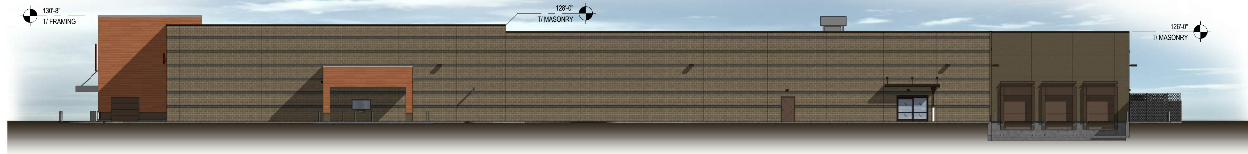
WEST ELEVATION
