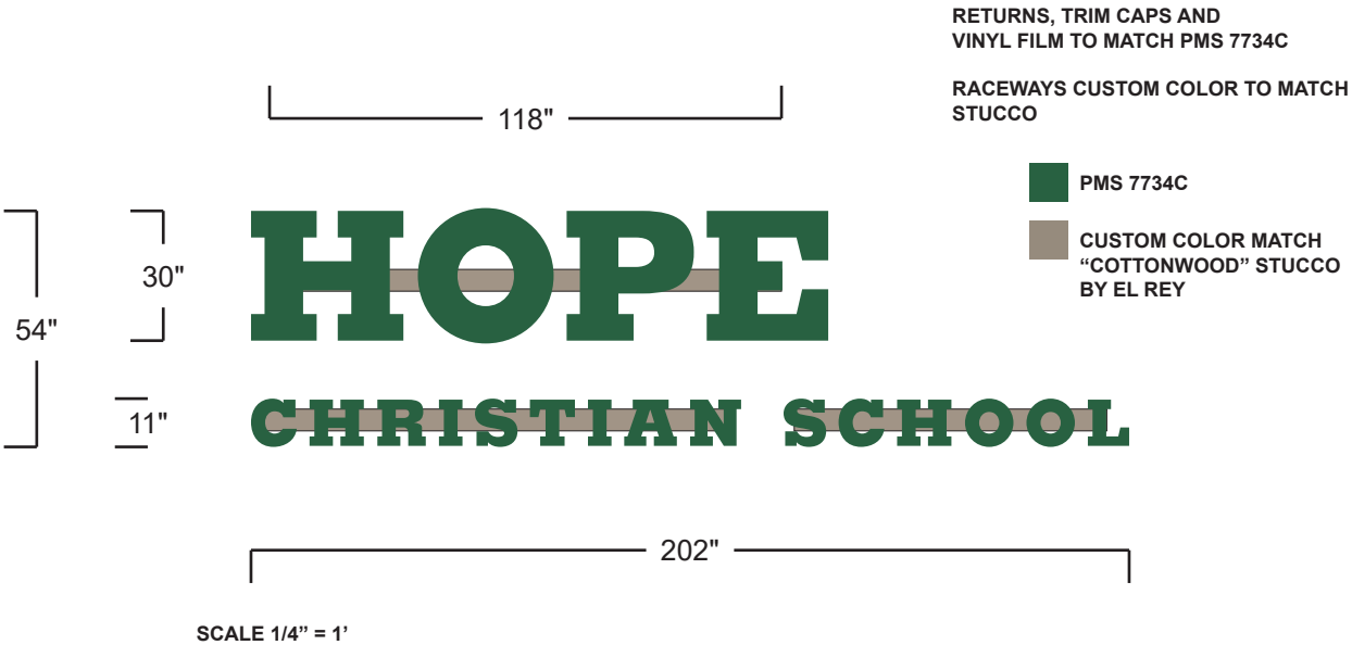
SCALE 1/4" = 1'
