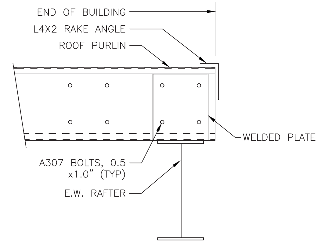
A7 SECTION THRU ENDWALL RAFTER
