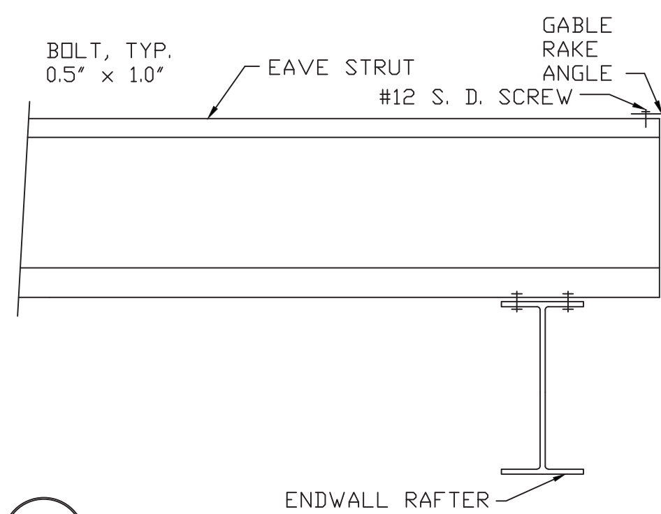
I8 EAVE STRUT TO ENDWALL RAFTER
