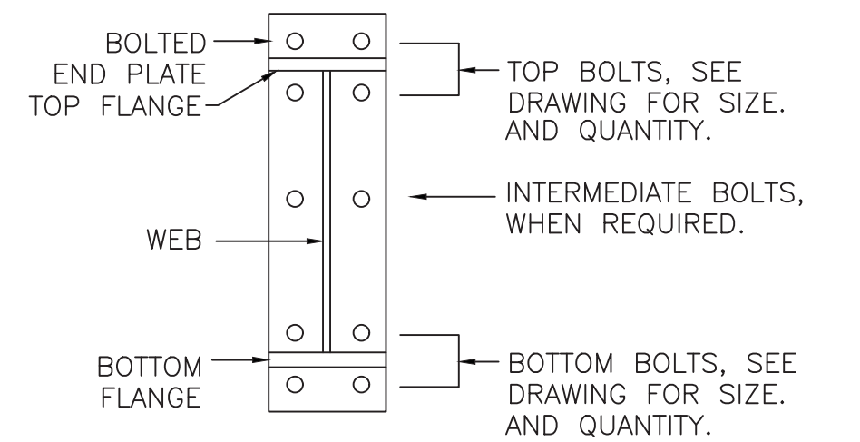
U3 BOLTS FOR RAFTER TO COLUMN CONNECTION
