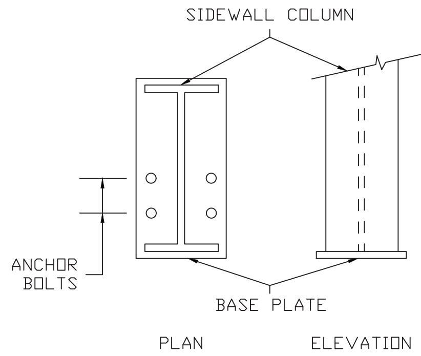
R2 ANCHOR BOLTS AT SIDEWALL COLUMN
