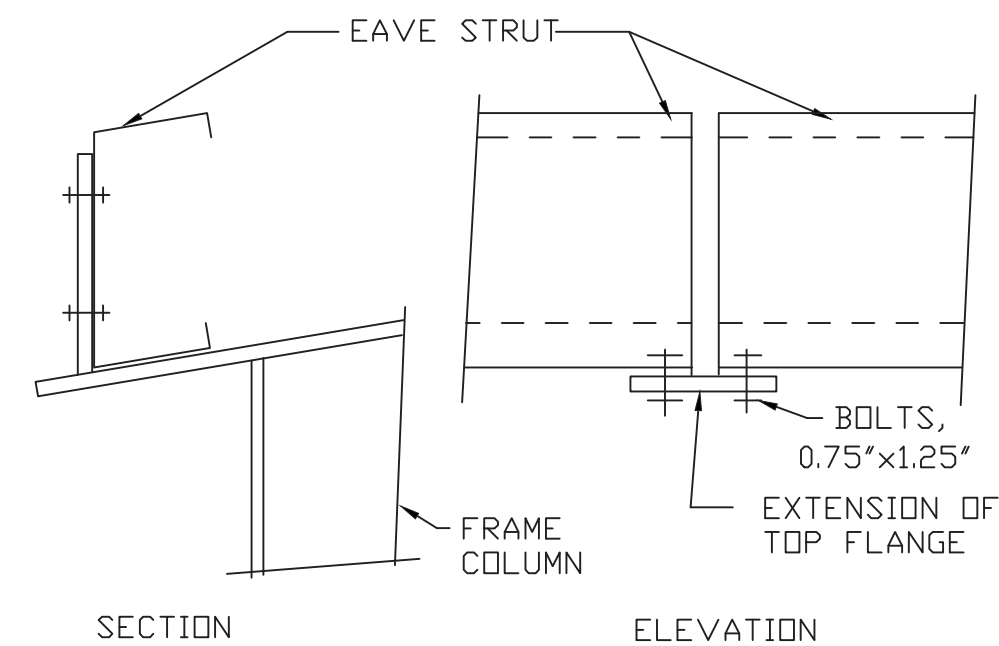
J2 EAVE STRUT TO RIGID FRAME
