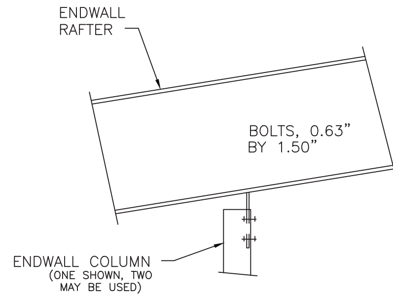
B4 ENDWALL RAFTER TO COLUMN
