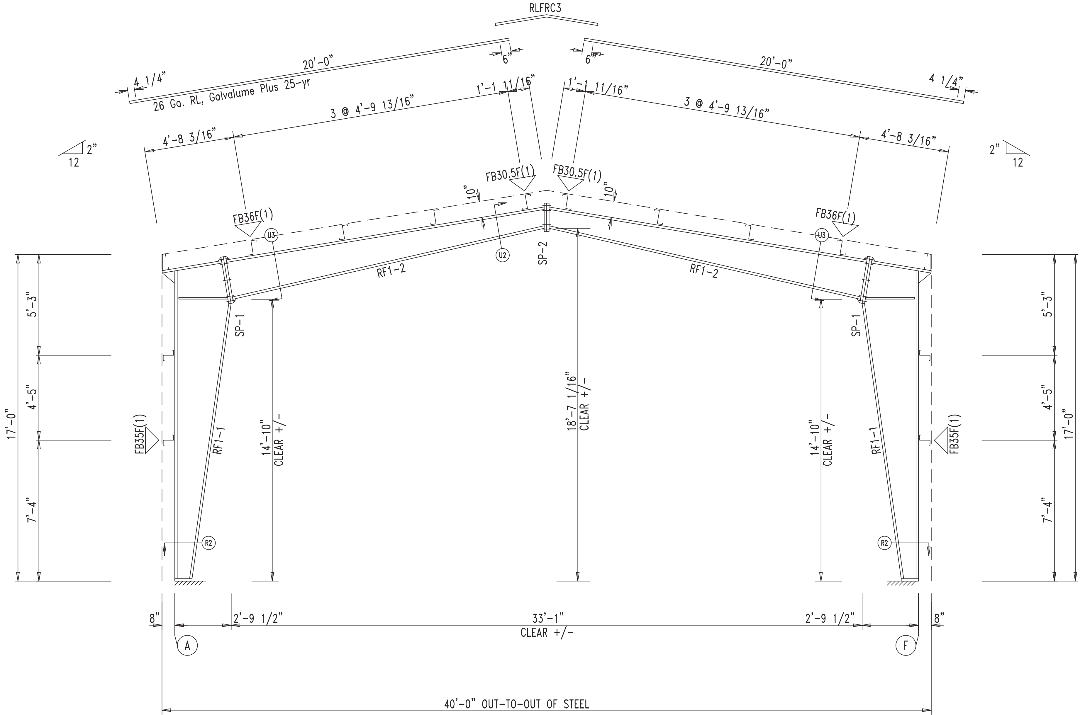
RIGID FRAME ELEVATION: FRAME LINE 2
