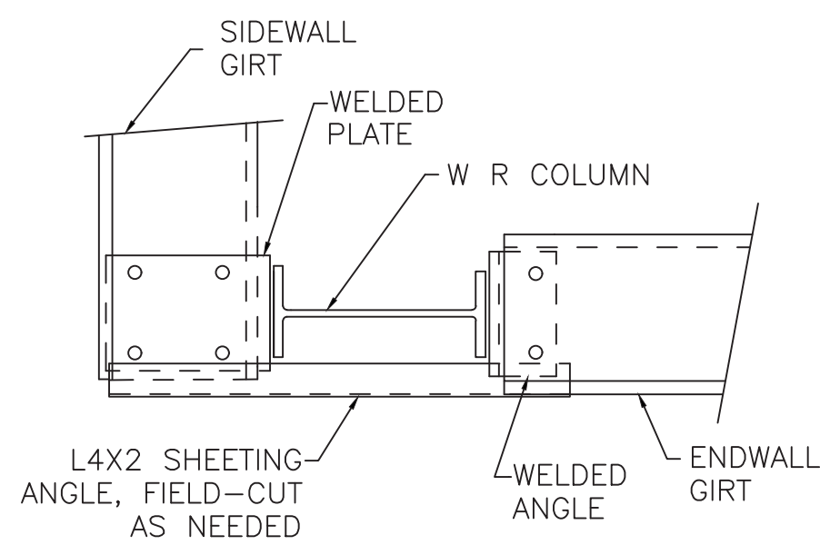
D17 CORNER COLUMN TO WALL GIRT
