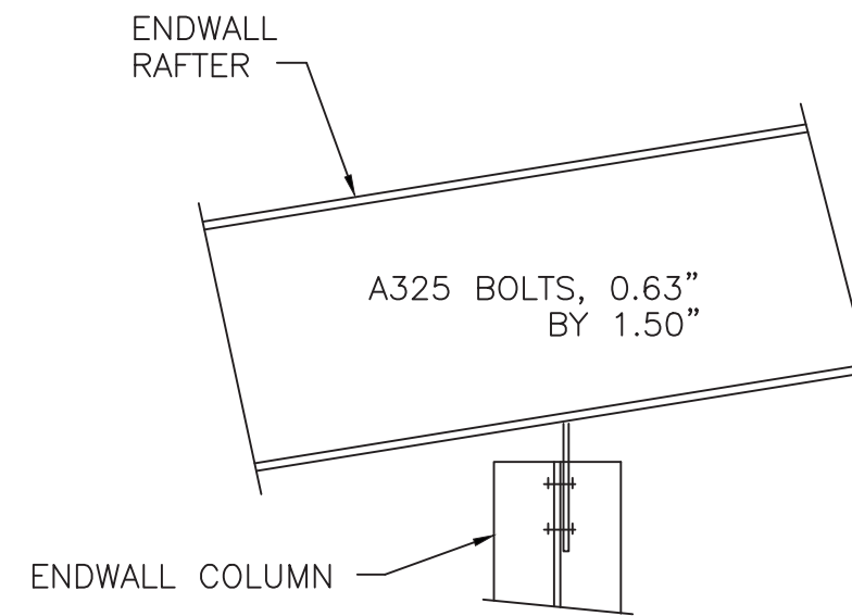
B6 ENDWALL RAFTER TO COLUMN
