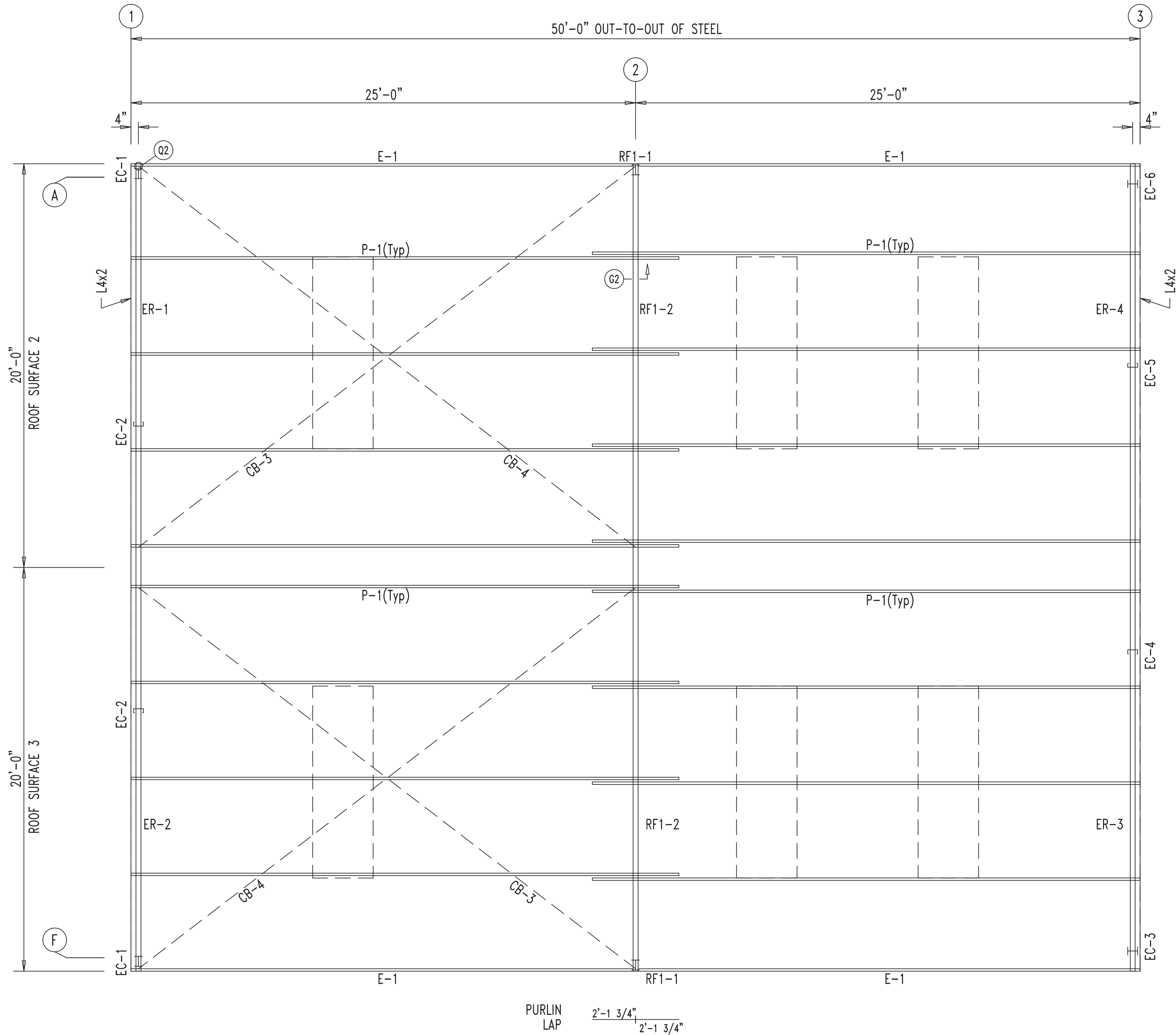
ROOF FRAMING PLAN
