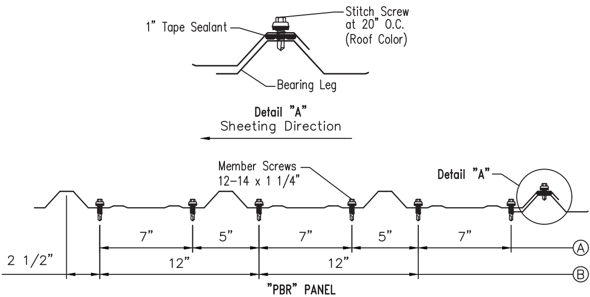
FASTENER LOCATION FOR ROOF PANELS
