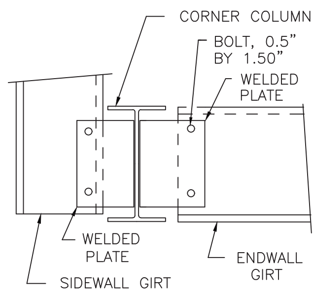
D6 CORNER COLUMN TO WALL GIRT
