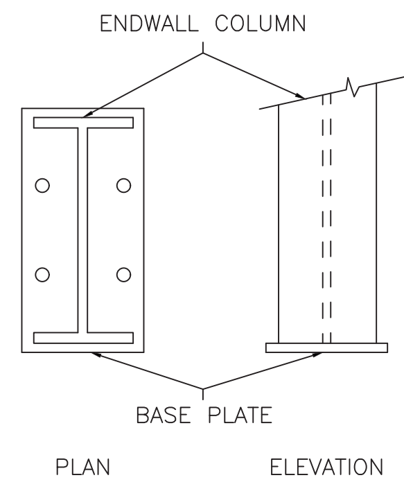
E3 BASE PLATE FOR ENDWALL COLUMN
