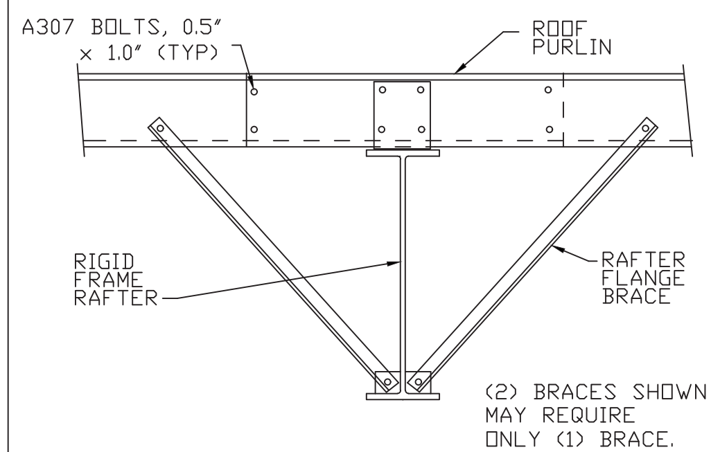
G2 ROOF PURLIN TO INTERIOR FRAME RAFTER
