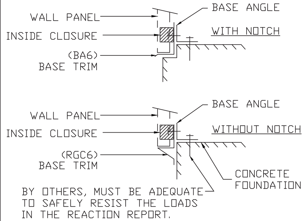
T1 SECTION THRU WALL PANEL AND CONCRETE FOUNDATION
