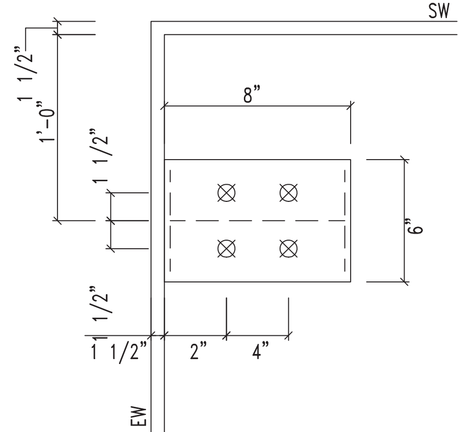
DETAIL B
