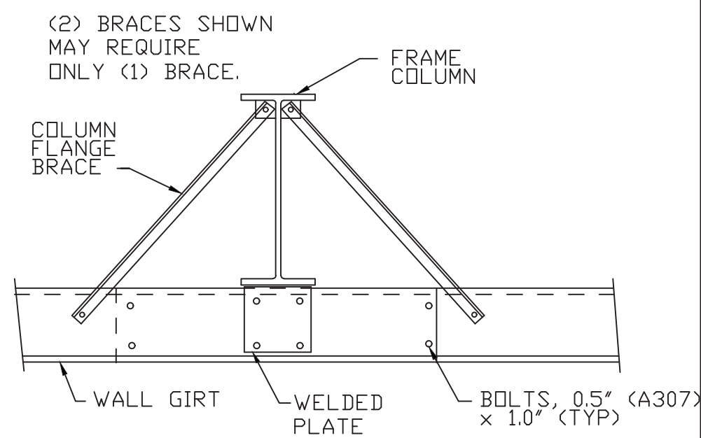
H2 WALL GIRT TO FRAME COLUMN
