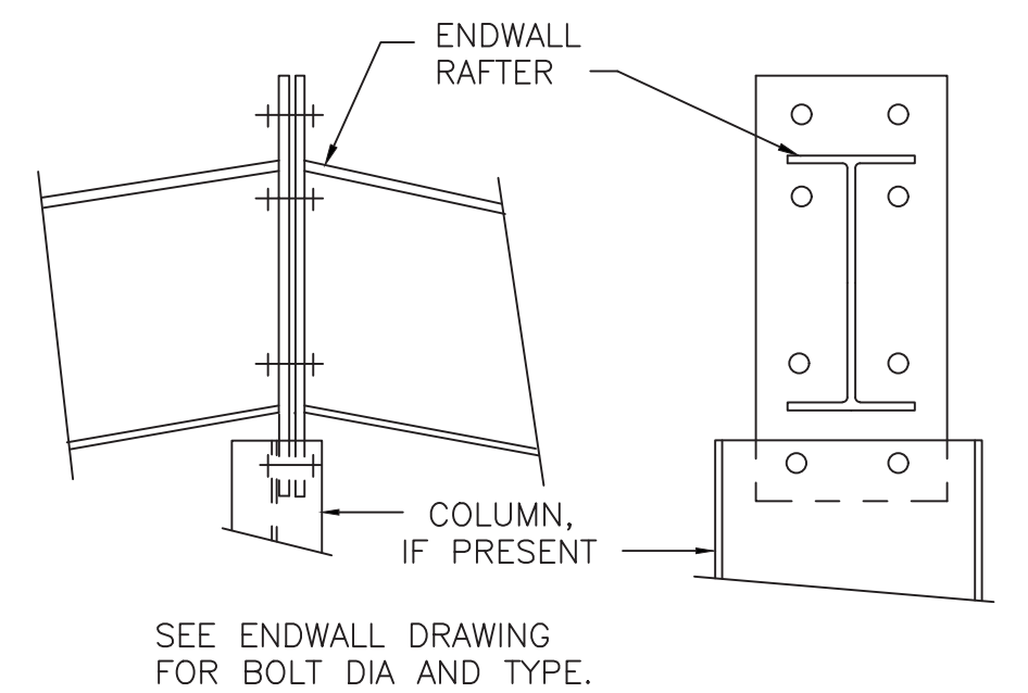
F12 RAFTER SPLICE AT SURFACE CHANGE
