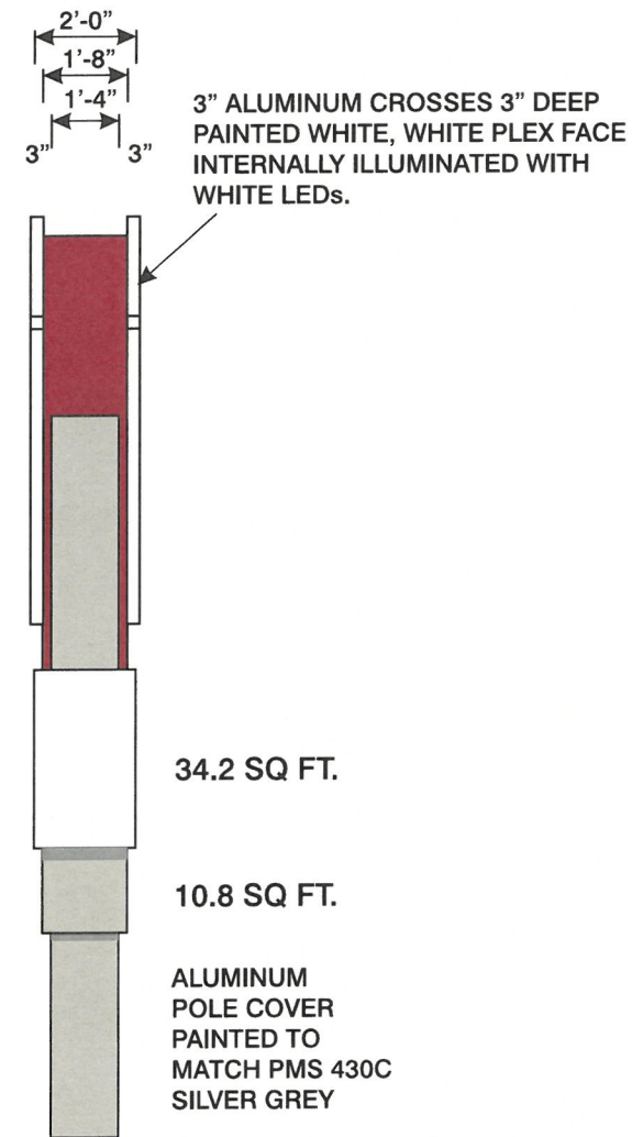
END VIEW
