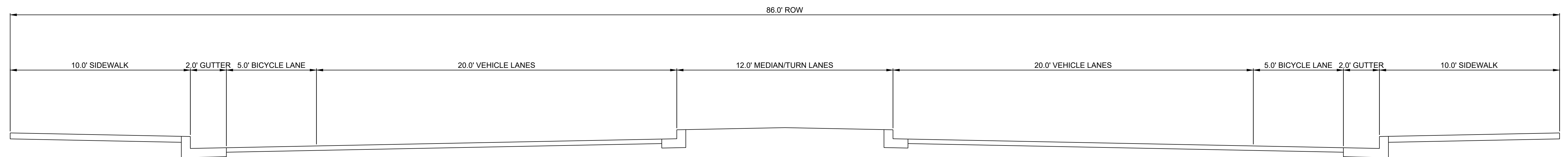
FUTURE SECTION WITH BICYCLE LANES OPTION #1 NTS
