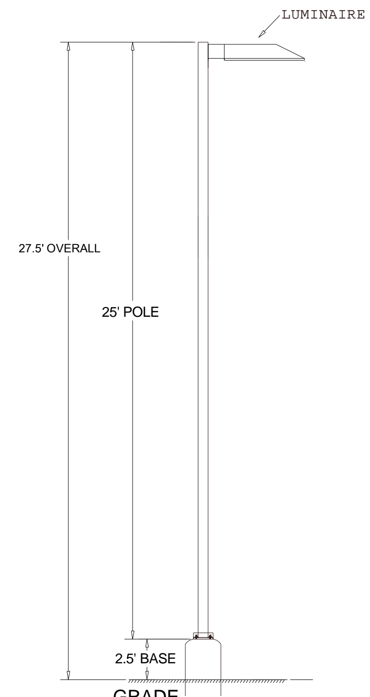
POLE DETAIL (NOT TO SCALE)
