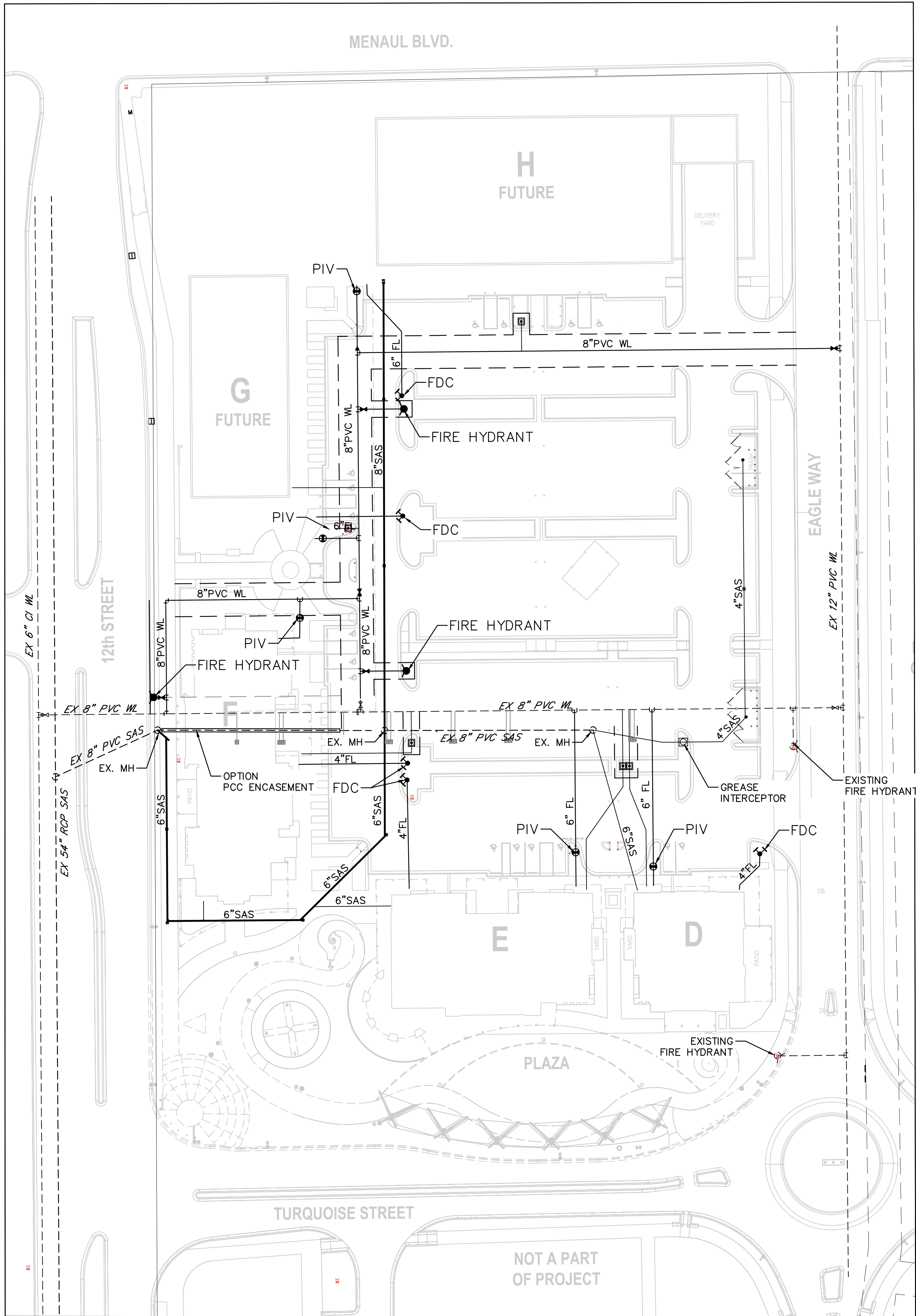
UTILITY PLAN
