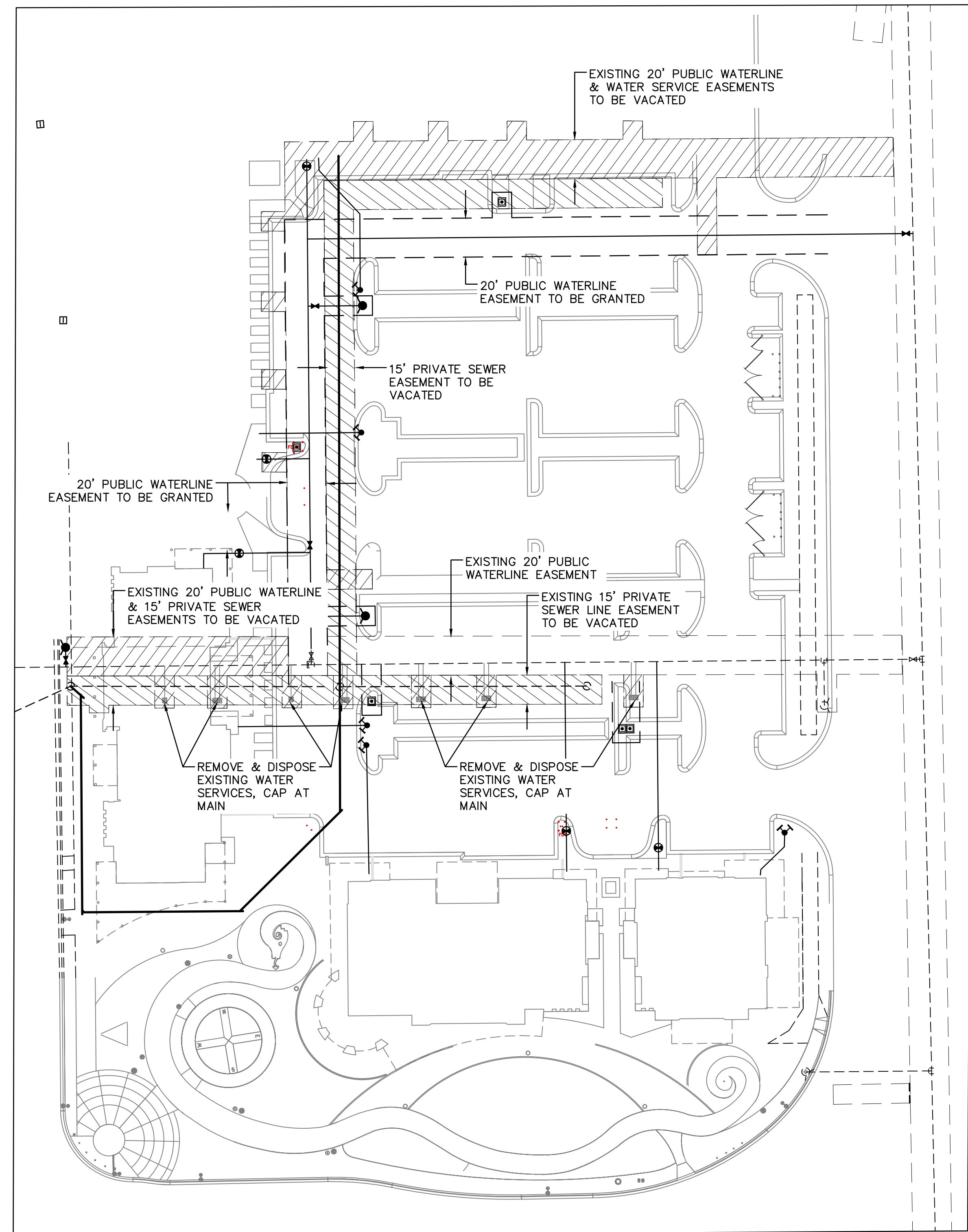
DEMOLITION & EASEMENT VACATION PLAN
