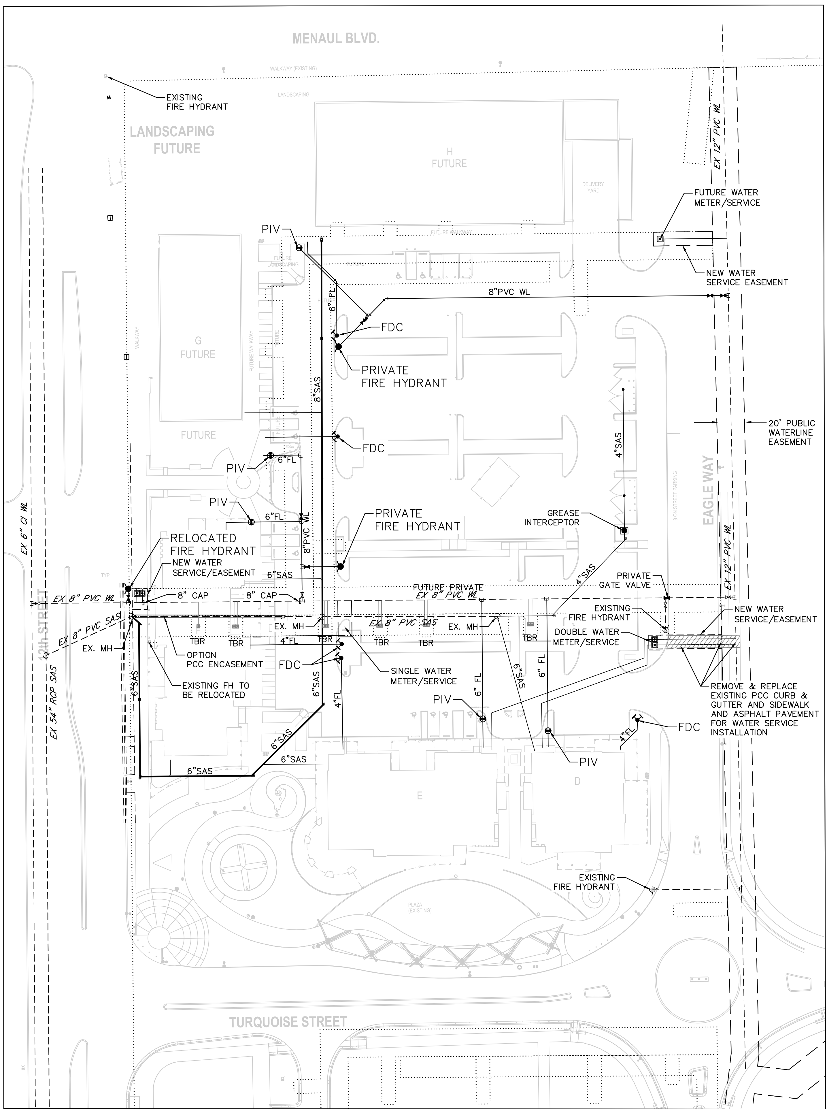
UTILITY PLAN
