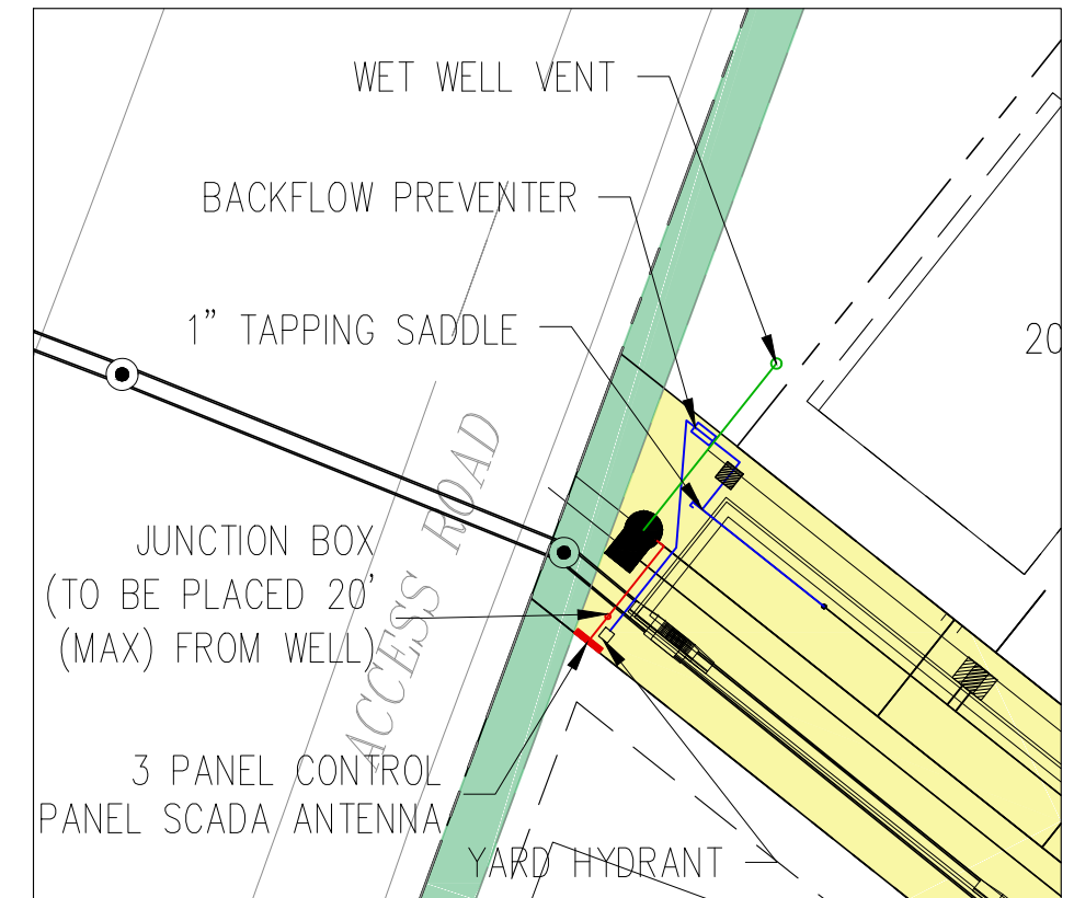
LIFT STATION SCALE: 1"=40'
