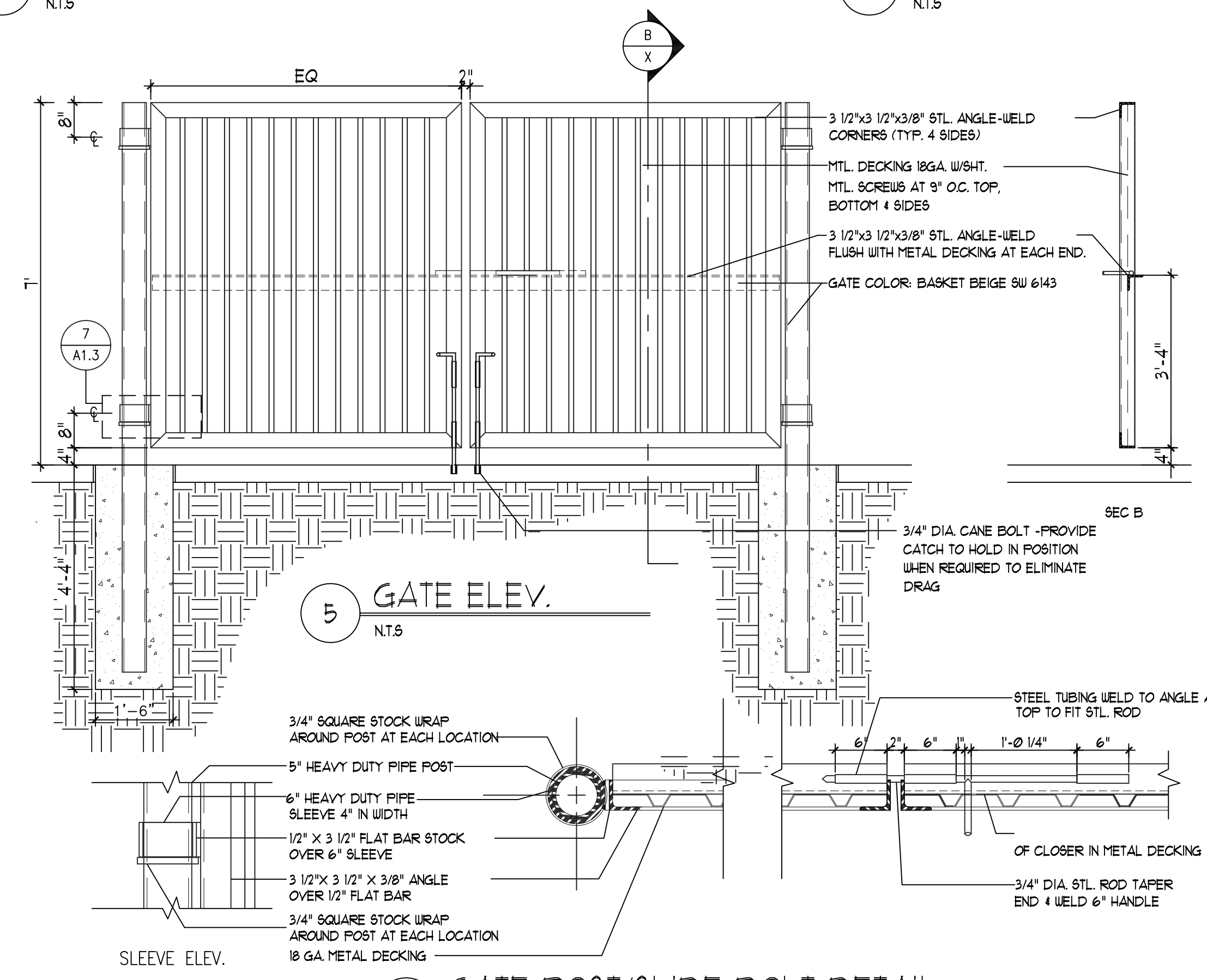
7 GATE POST/SLIDE BOLT DETAIL NTS
