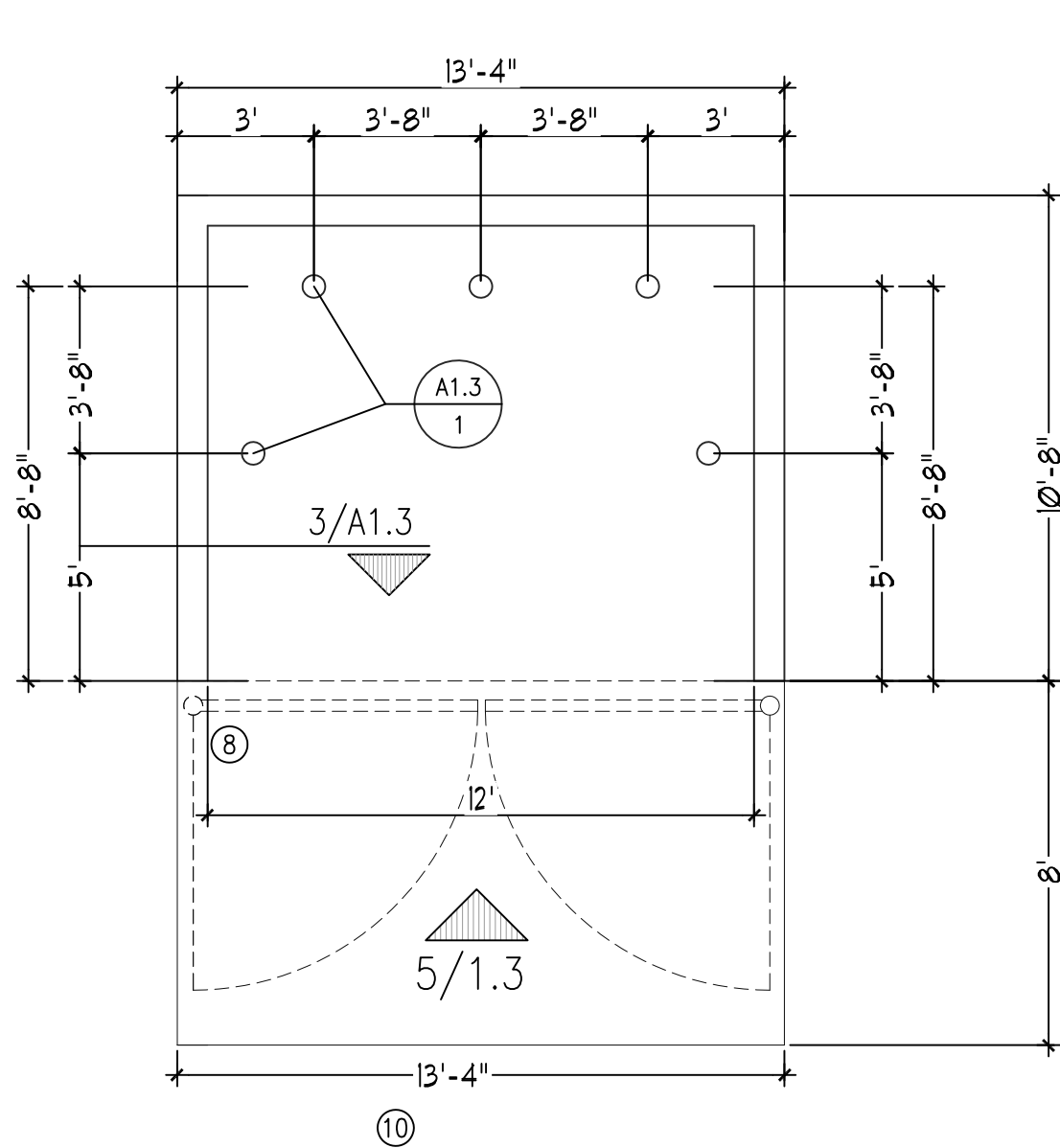
4 DUMPSTER PLAN NTS
