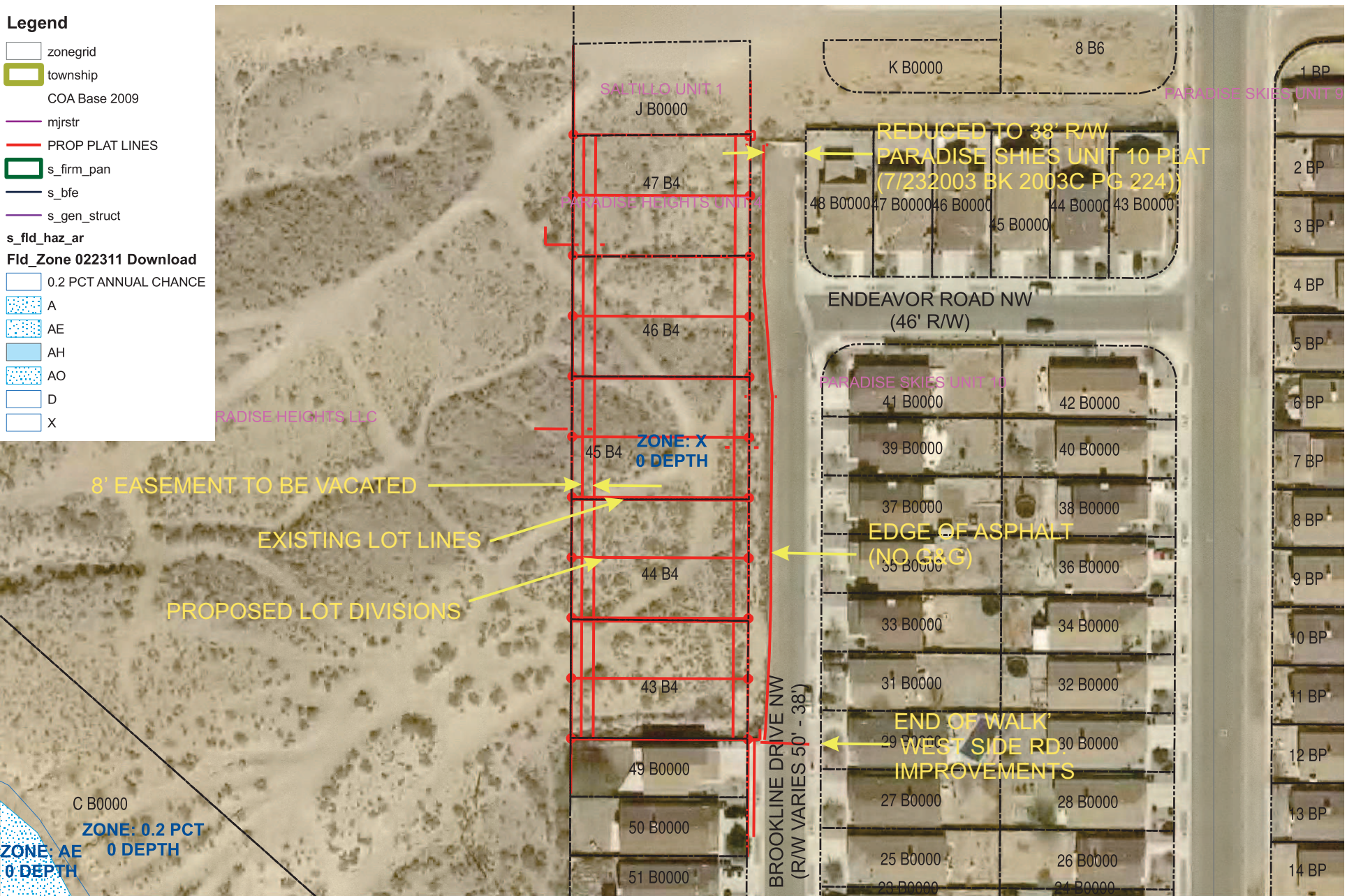
PARADISE HEIGHTS UNIT 4, BLOCK 4, LOTS 43 - 47 - PROPOSED REPLAT EXHIBIT INCLUDES VACATION OF 8' CONSTRUCTION AND UTILITY EASEMENT OVERLOOKED IN PROJECT 1002379 (2002 DRB) FILED 05/07/1968 BK D3 PAGE 201
