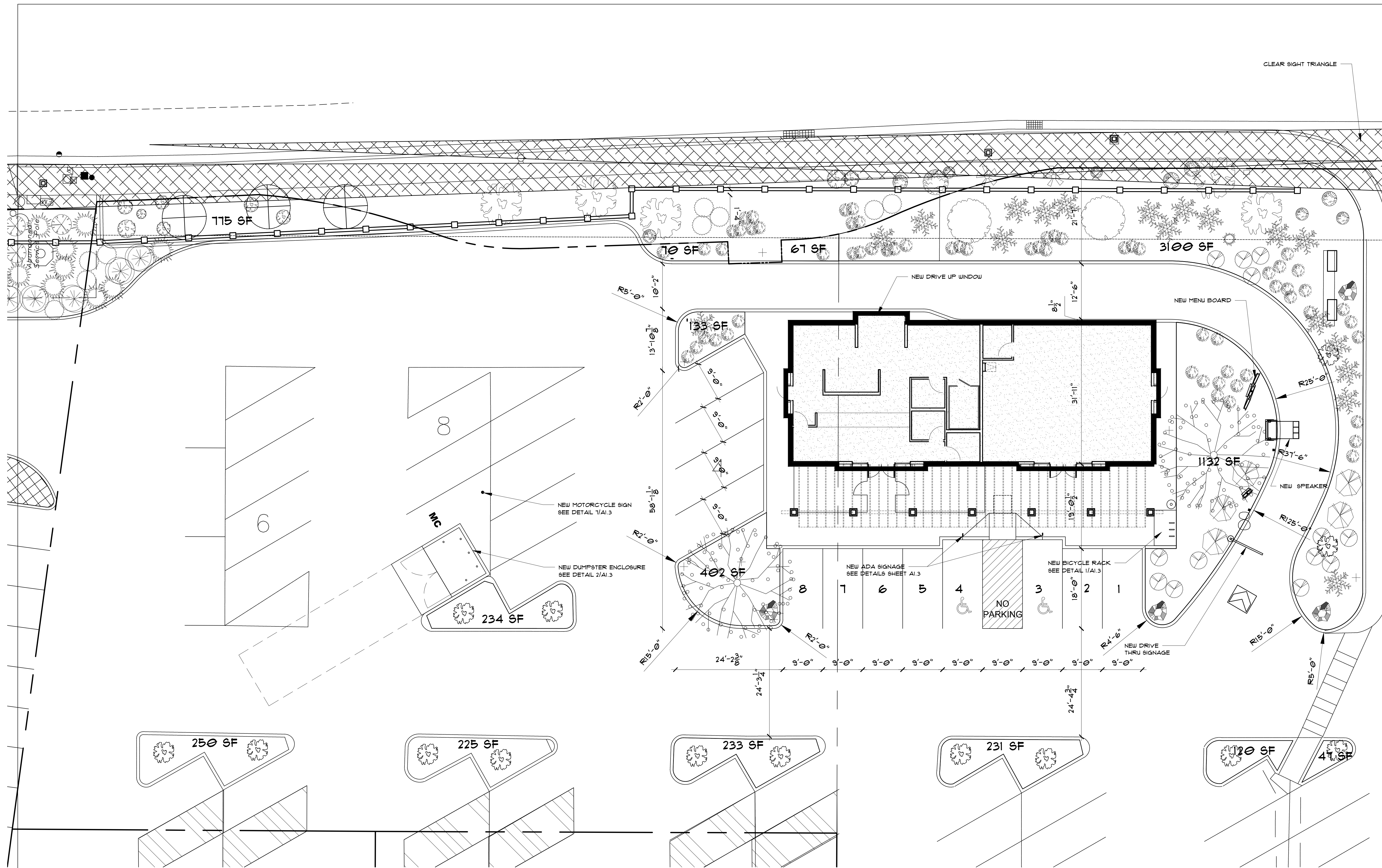
ENLARGED SITE PLAN 1" = 10'-0"
