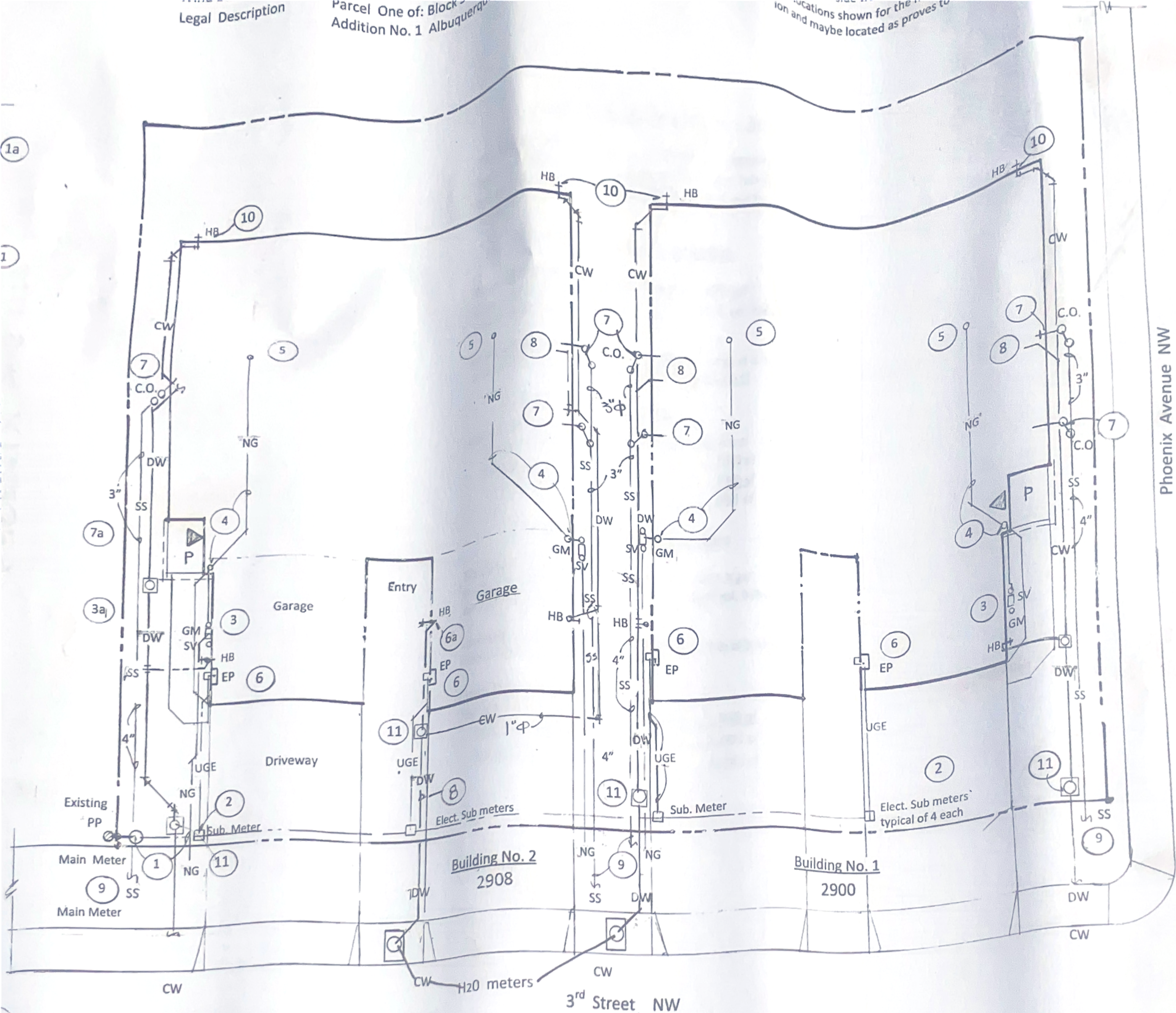
Site Utilities Plan Scale: 1" 10'-0"
