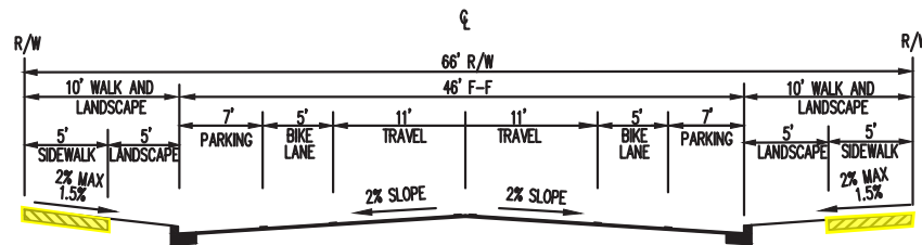
TYPICAL STREET SECTION -DEKOONING AVE CONNECTOR RESIDENTIAL 66' ROW
