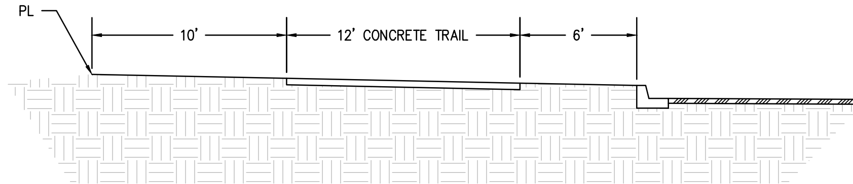
1 UNSER BLVD. 150' ROW Scale: 1"=5'
