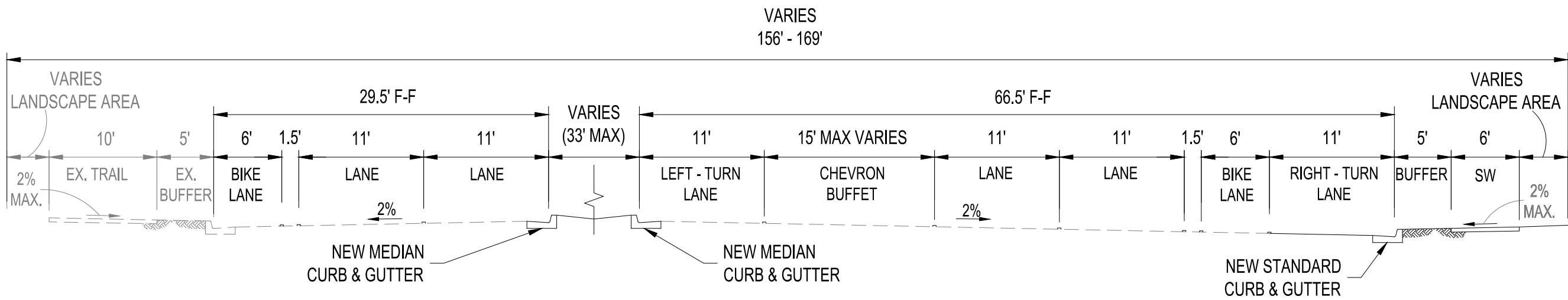
STREET SECTION B-B NOT TO SCALE
