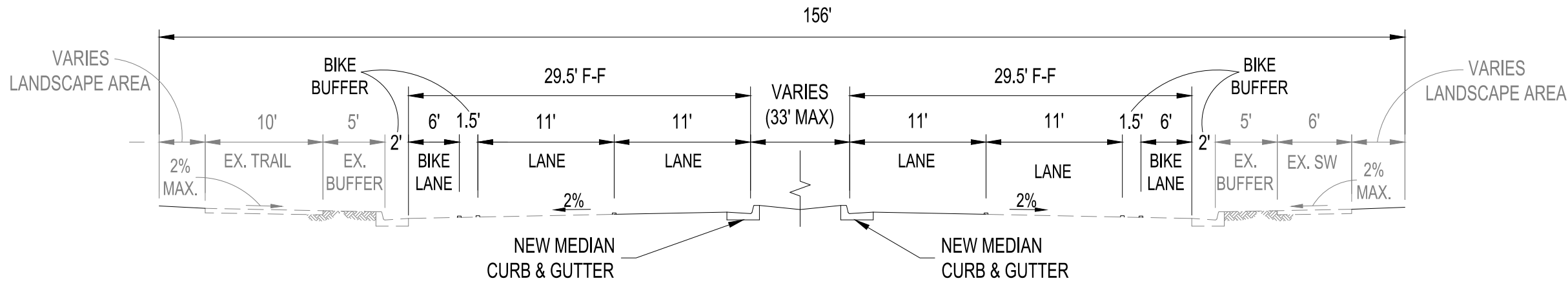
STREET SECTION A-A NOT TO SCALE
