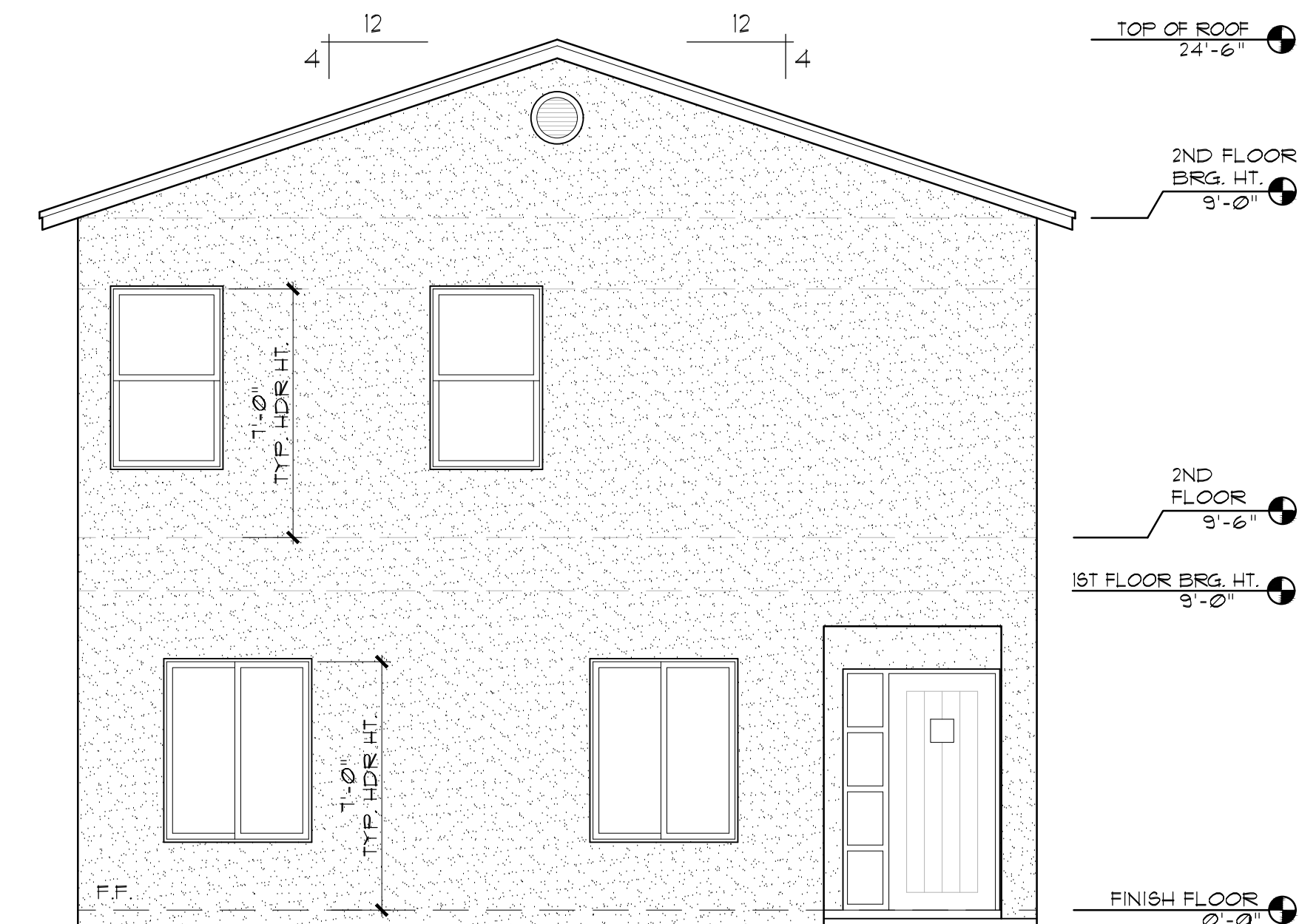
EAST ELEVATION
