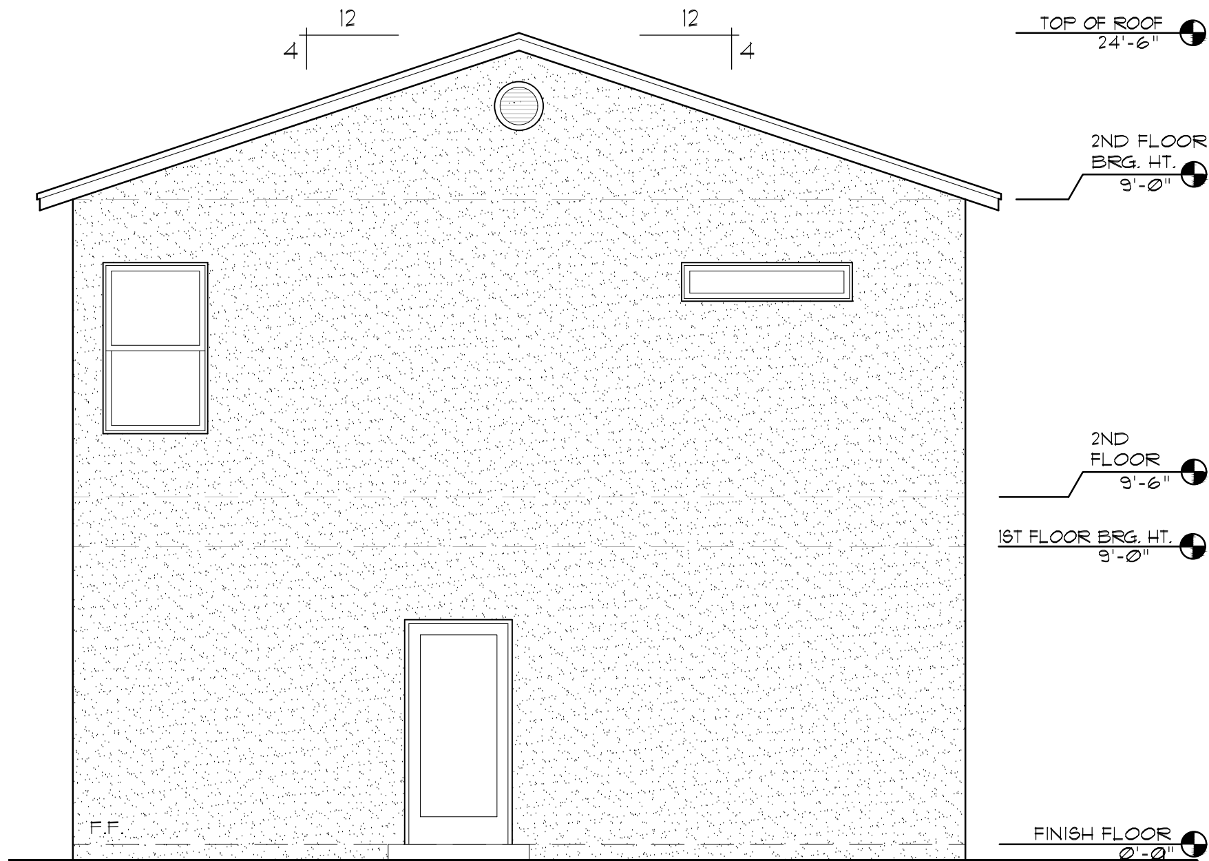
WEST ELEVATION
