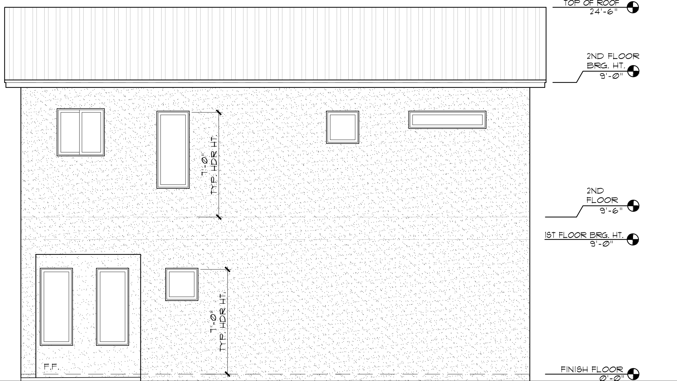
EAST ELEVATION
