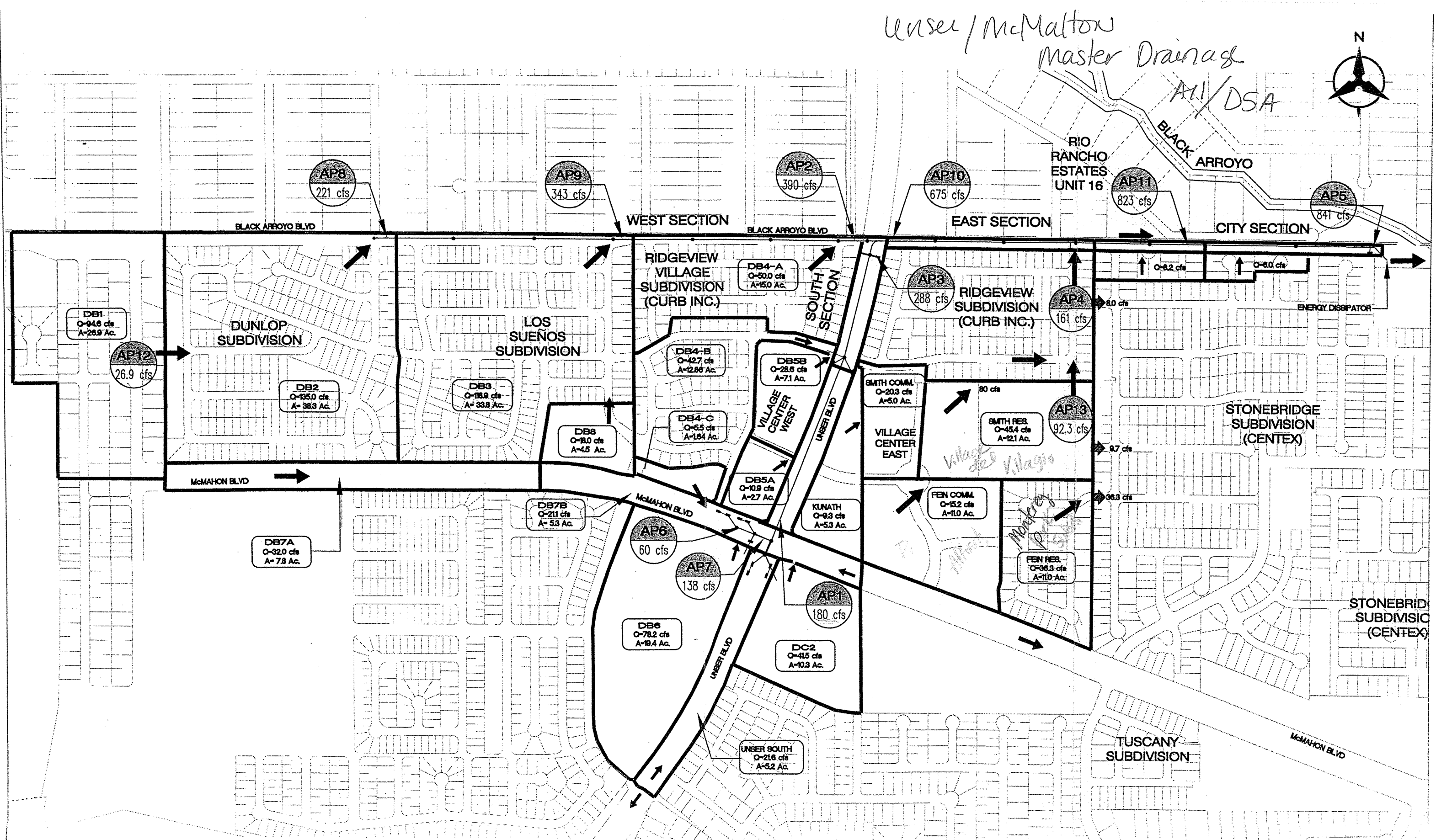
FIGURE 2 DEVELOPED CONDITIONS BASIN MAP
