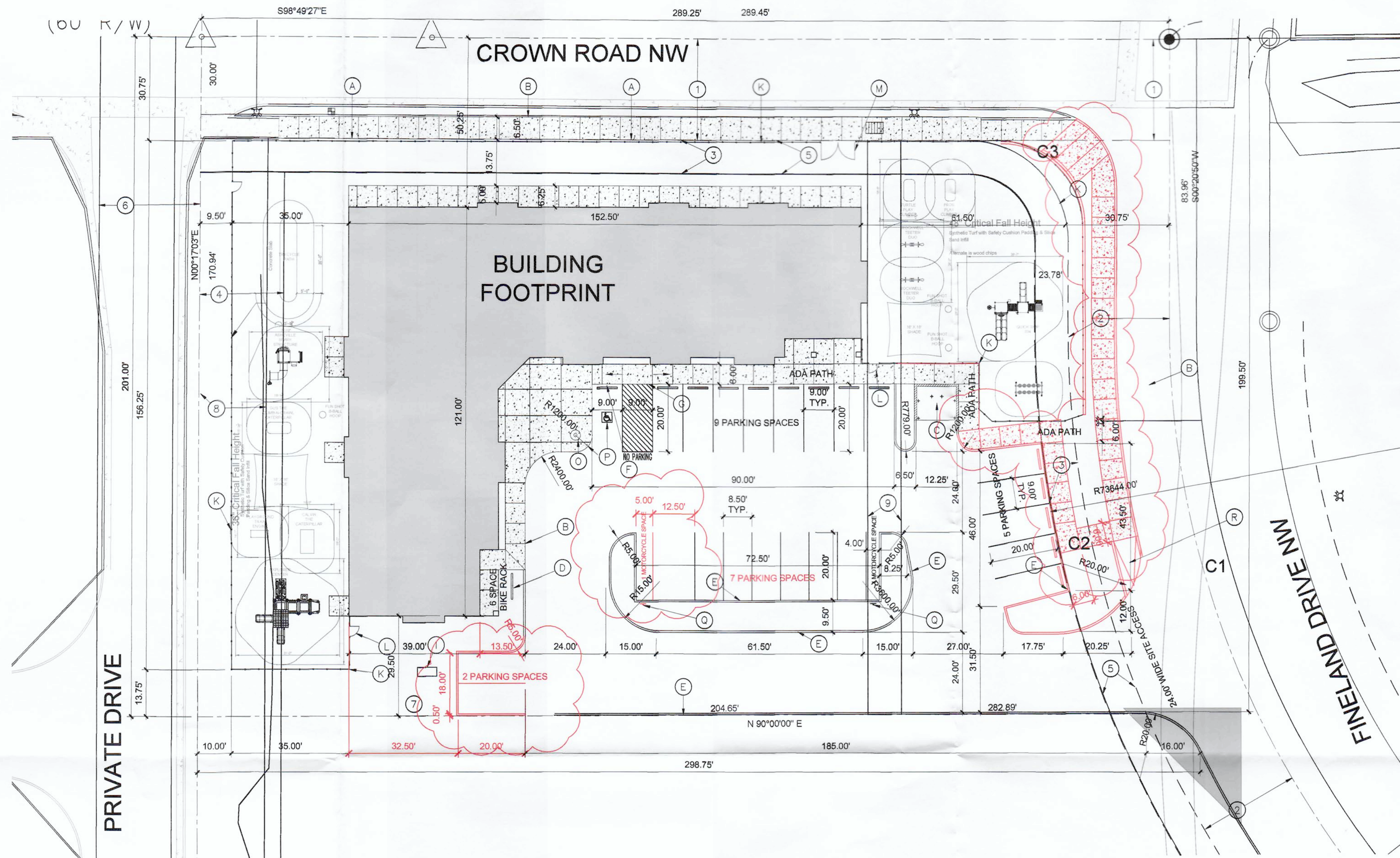
SITE PLAN
