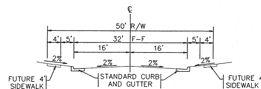
TYPICAL STREET SECTION A-A NO SCALE
