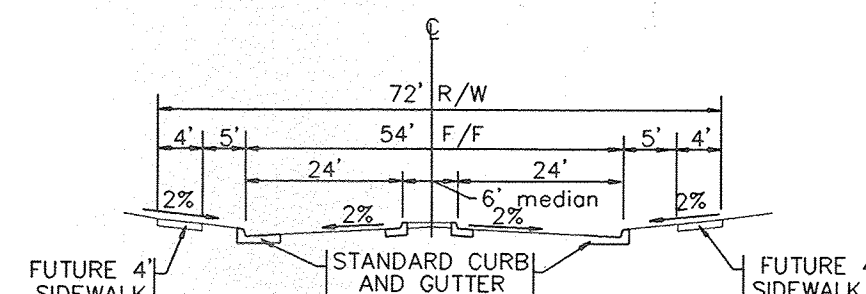
ENTRY STREET SECTION A-A NO SCALE
