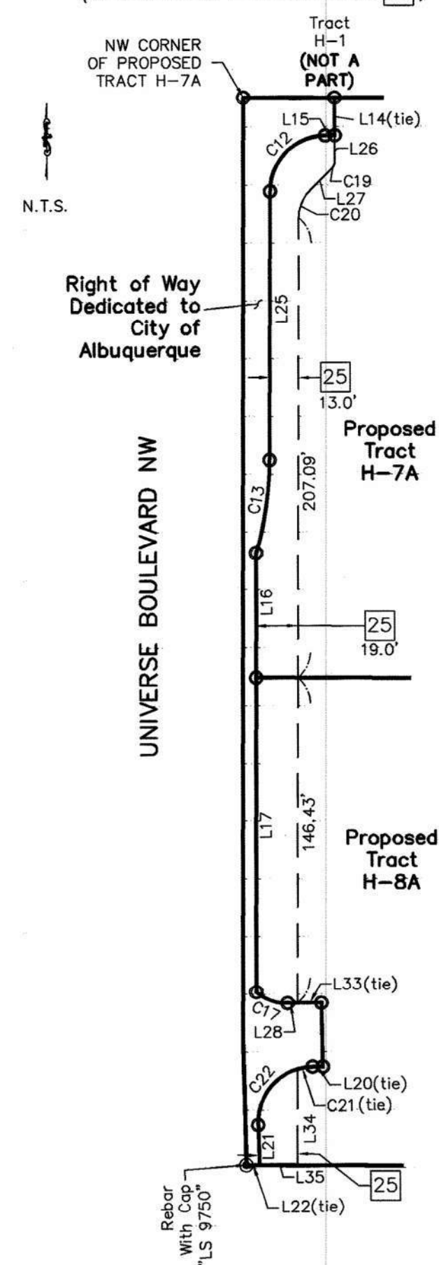
Detail "A" (Detail for Easement [25])
