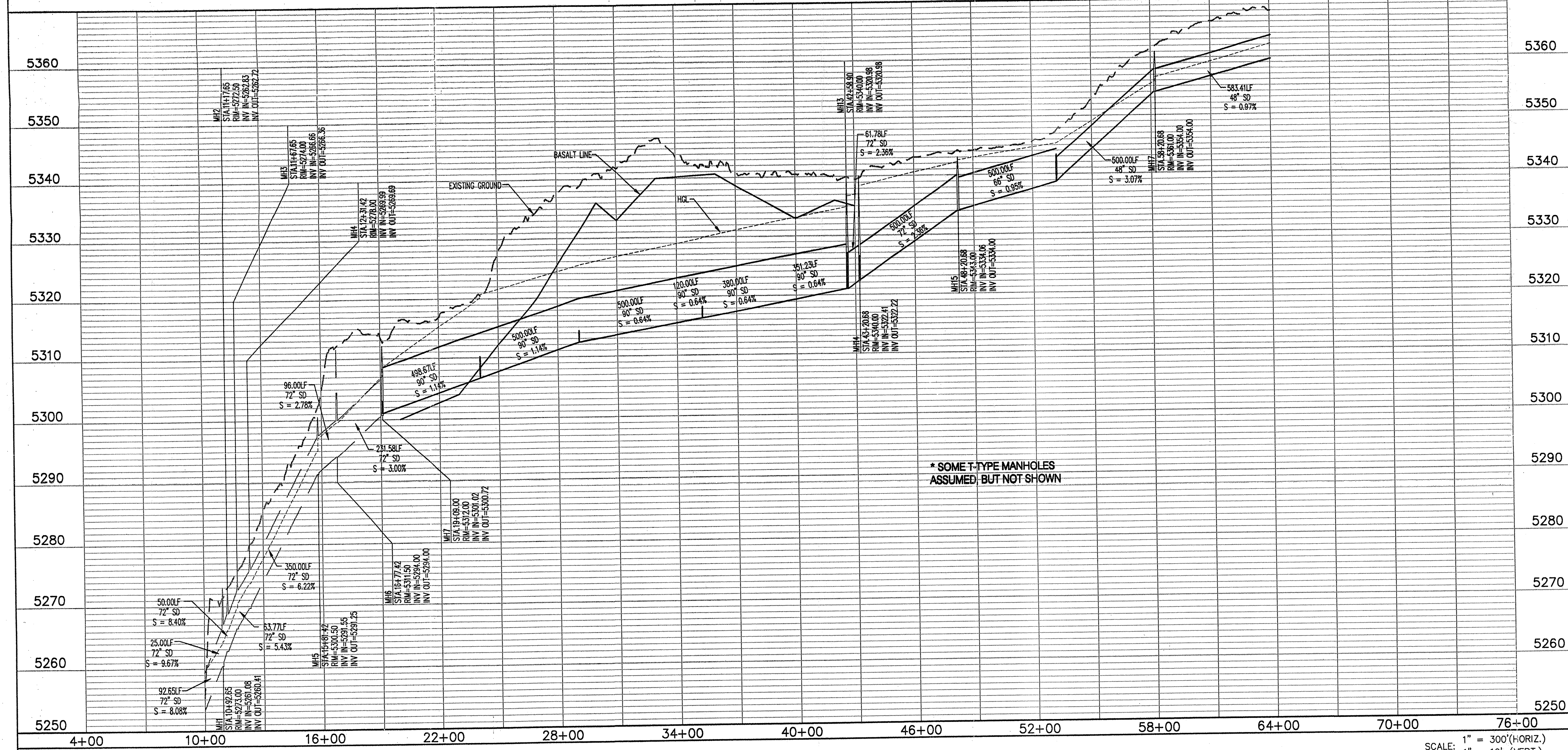
OPTION #4 PLAN & PROFILE
