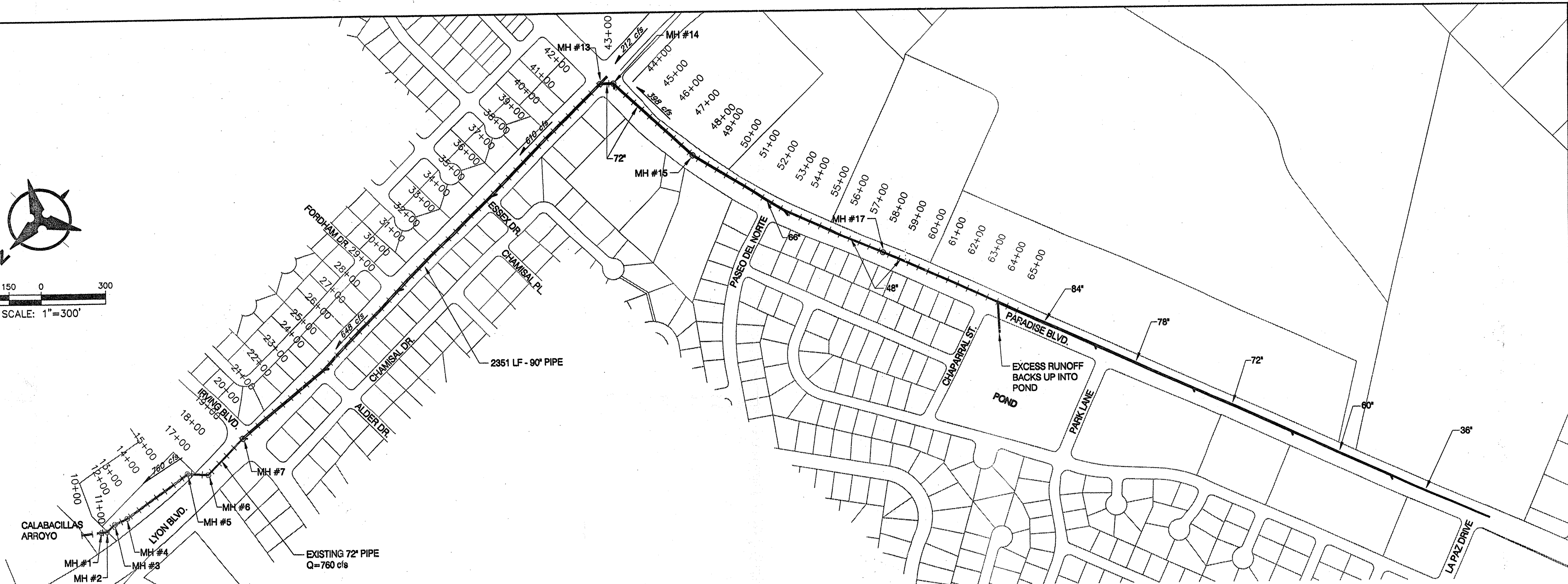
OPTION #4 PLAN & PROFILE
