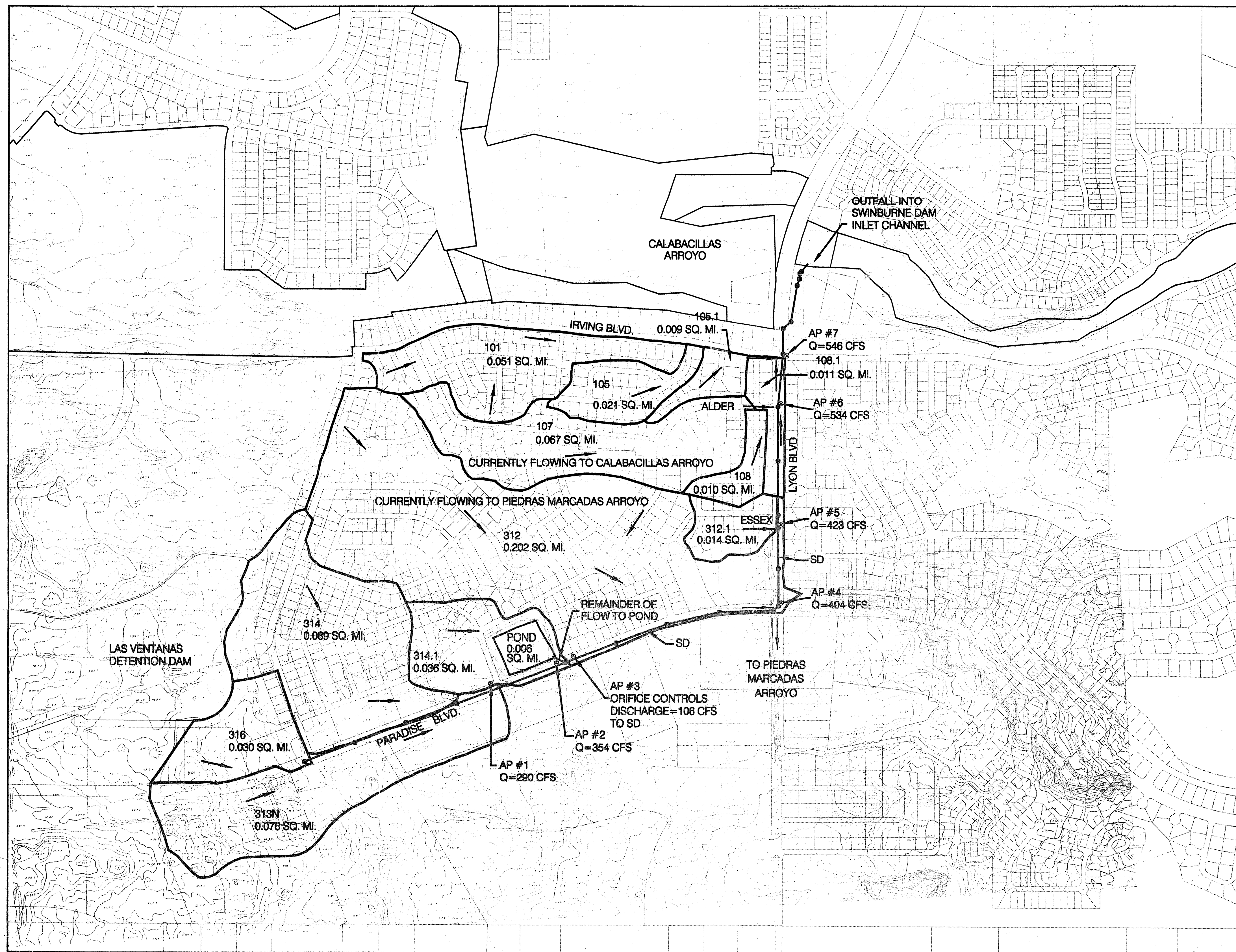
DRAINAGE BASIN MAP
