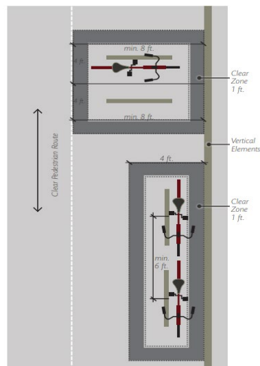
FIGURE 7.4.115 Bicycle Parking Stall Layout Options
