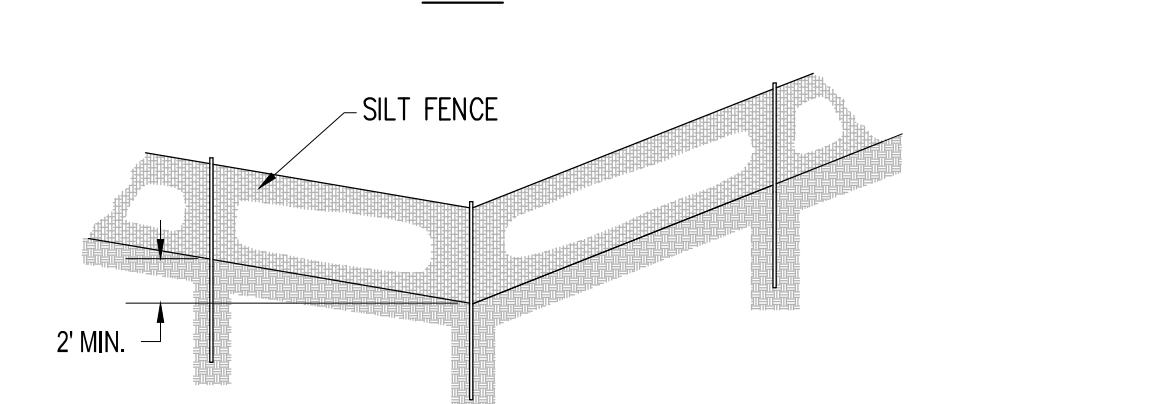
SILT FENCE DETAIL NOT TO SCALE
