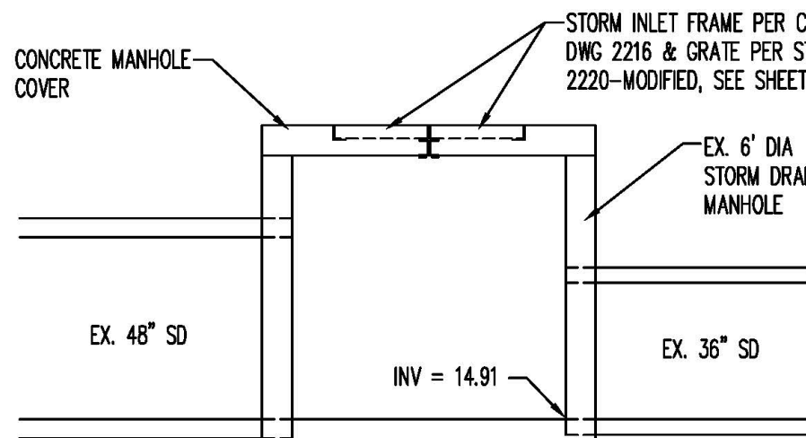
ELEVATION VIEW
