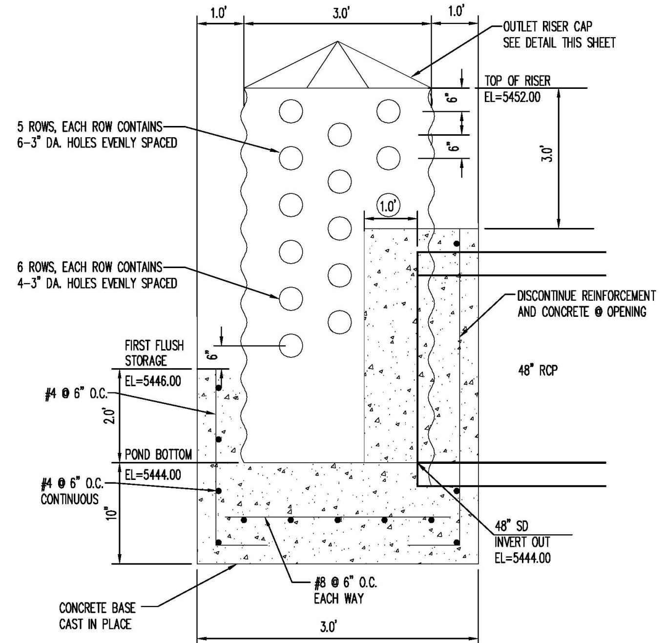
POND OUTLET RISER DETAIL NOT TO SCALE
