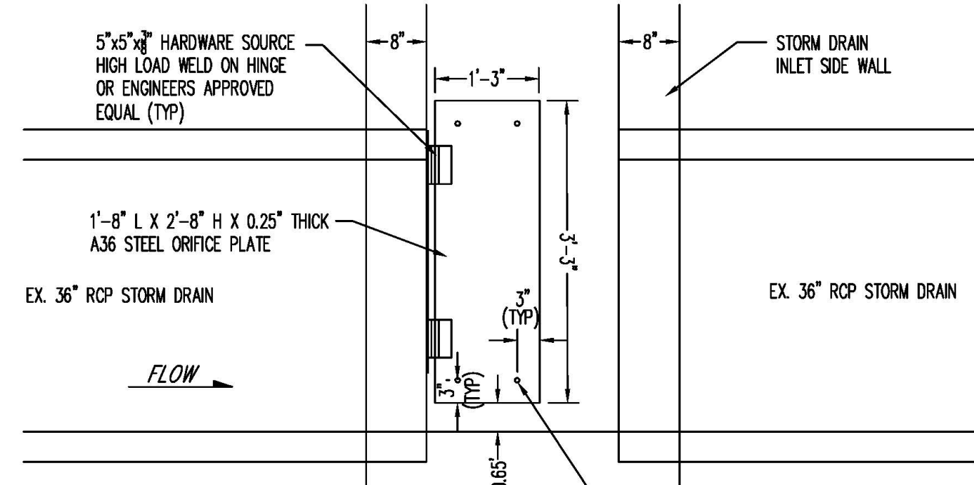
SIDE WALL STEEL ANCHOR PLATE
