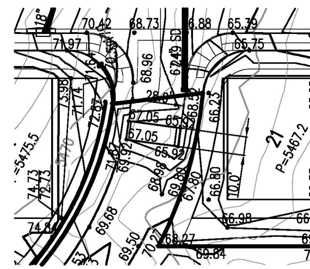
SANDMARK ROAD SEDIMENTATION POND SCALE: 1" = 50'
