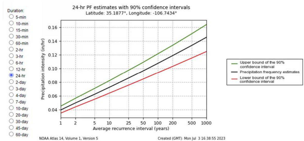
Figure 1.11 Intensity-Duration-Frequency Graph
