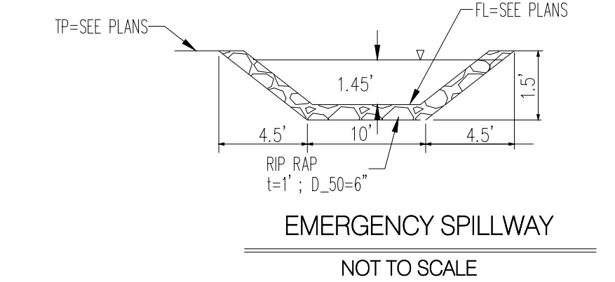
EMERGENCY SPILLWAY NOT TO SCALE
