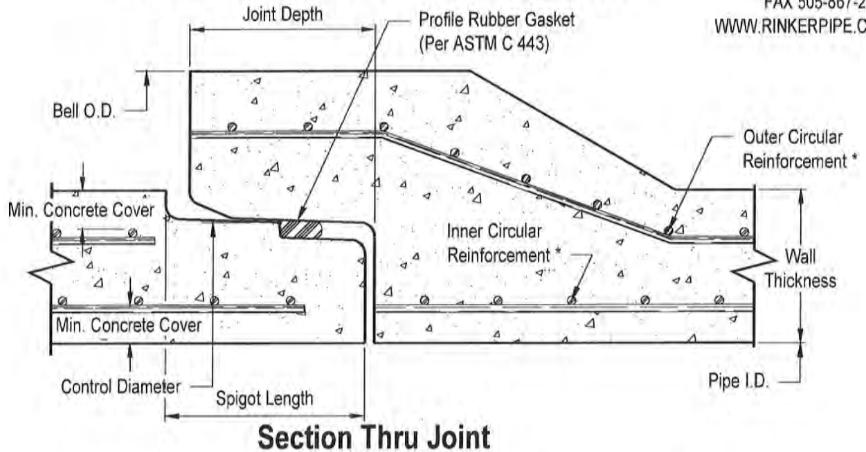
30"Ø to 72"Ø RCP (Big Bell Single Offset Joint) w/ Double Cage Reinforcement
