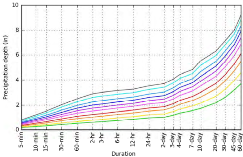
PDS-based depth-duration-frequency (DDF) curves Latitude: 35.1858°, Longitude: -106.7518°
