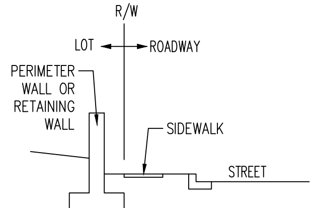
TYPICAL CROSS SECTION F-F NOT TO SCALE
