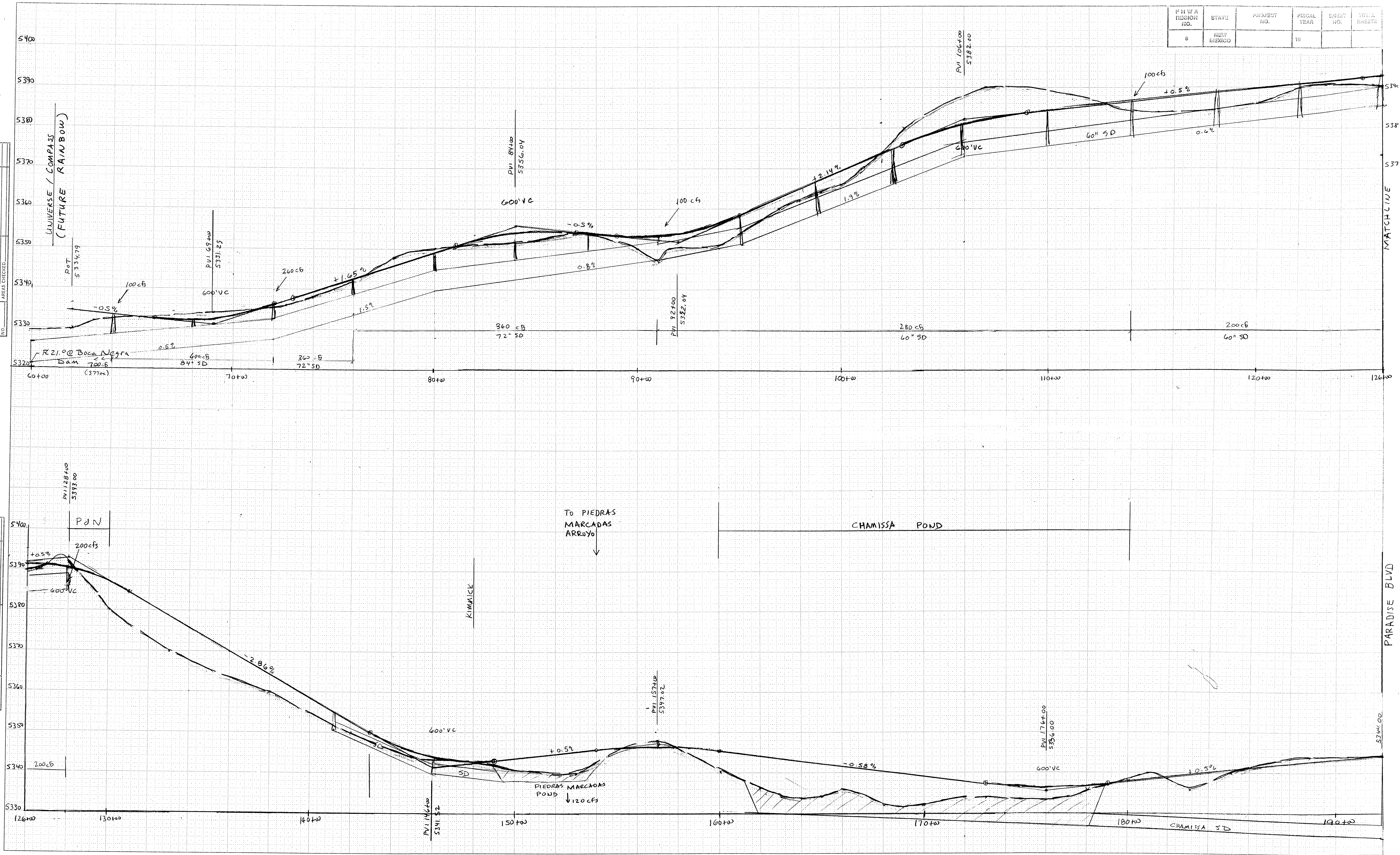
PLATE 1 CONCEPTUAL UNSER BLVD. PROFILE PARADISE BLVD. TO RAINBOW BLVD.
