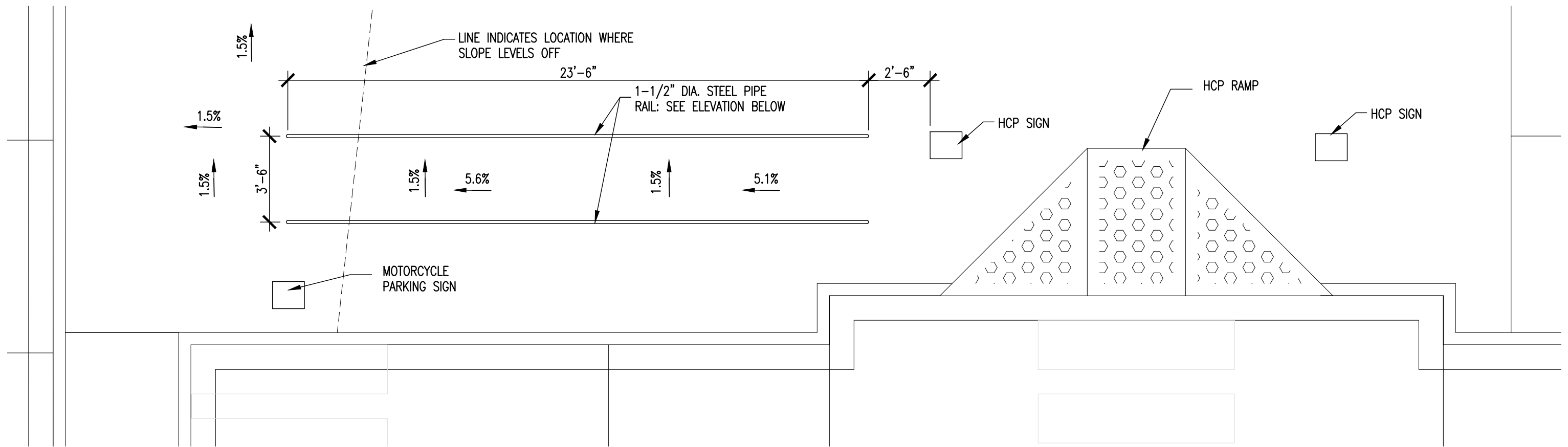
1 | partial courtyard and proposed ramp plan
