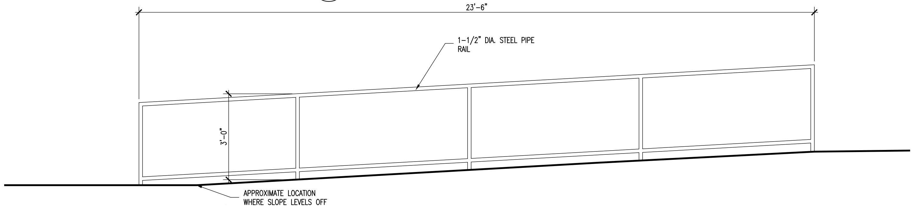
2 | handrail elevation
