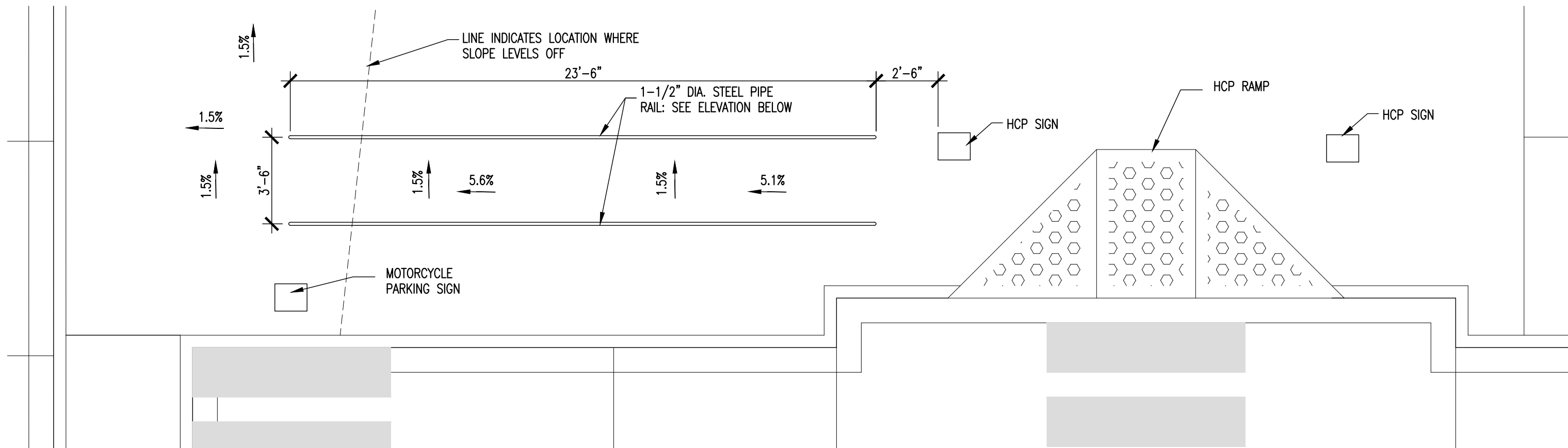
1 | partial courtyard and proposed ramp plan 1/4" = 1'-0"
