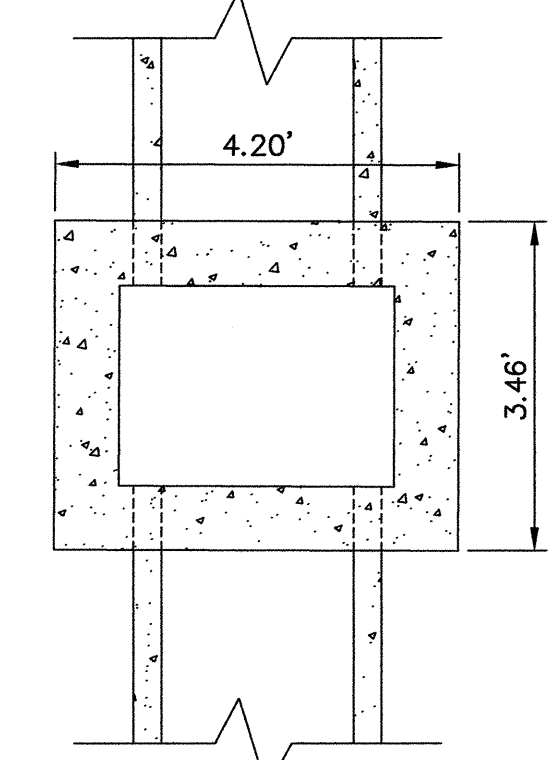
TYPE "D" STORM INLET DETAIL NTS
