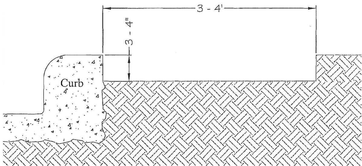
CUT BACK CURB DETAIL NOT TO SCALE
