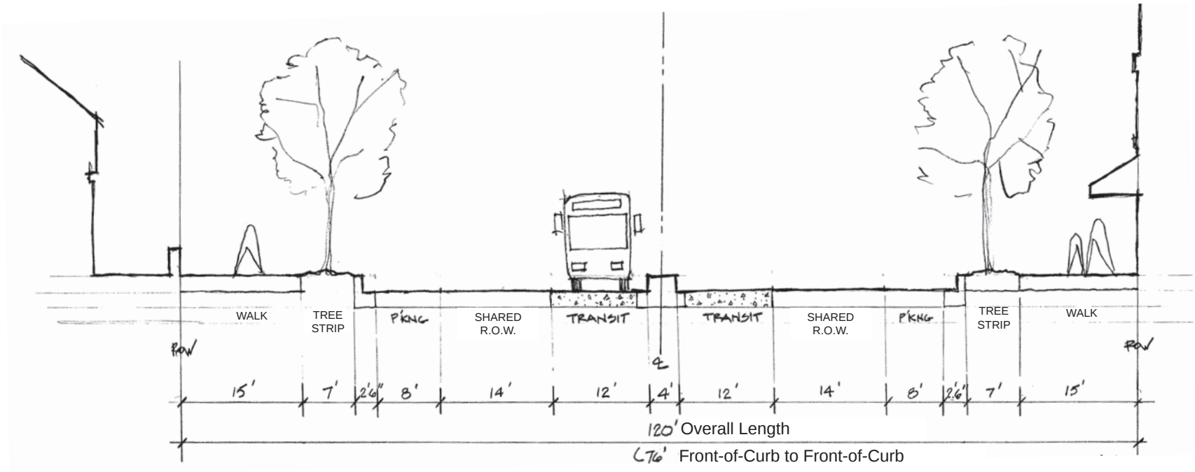
Cross Section 10 – Transit Boulevard Through Town Center
