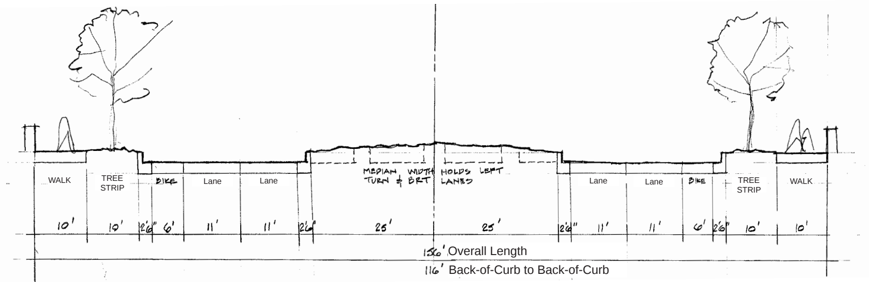
Cross Section 2, Urban Boulevard – Paseo del Norte & Unser Blvd. (no access/frontage lanes)
