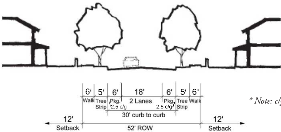
Cross Section 11 – Local Street
