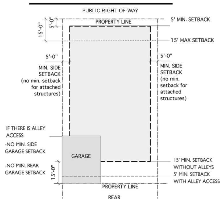
Figure 4, SU-2/VCUR Building Placement Diagram
