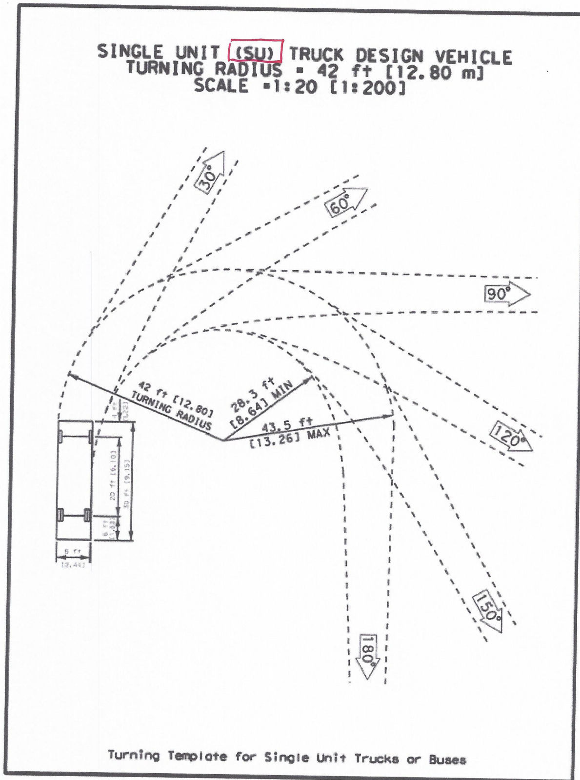
Figure 7-1. Turning Template for Single Unit Trucks or Buses, (not to scale).
