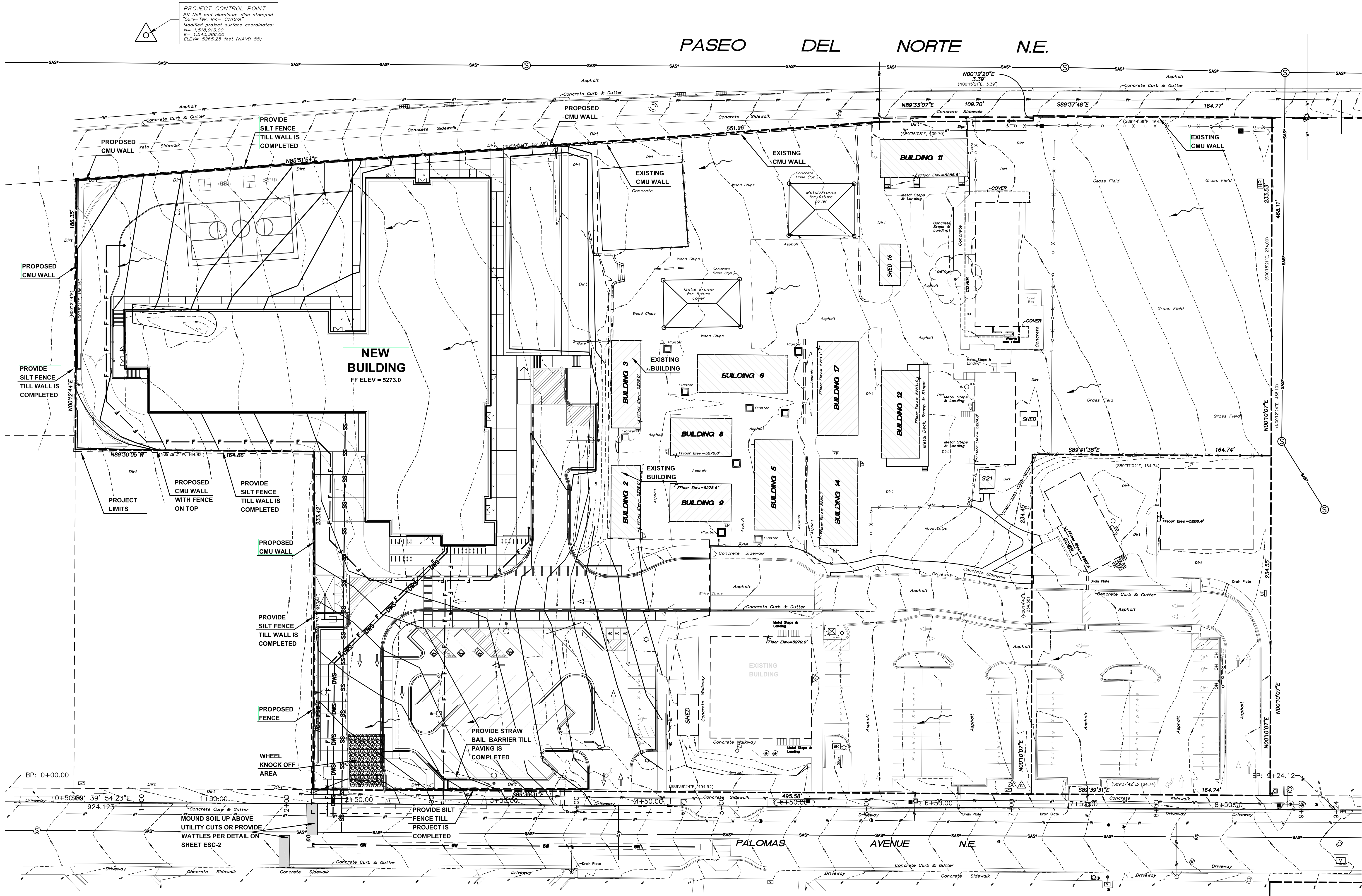
1 EROSION AND SEDIMENT CONTROL - PROPOSED CONDITIONS 1" = 30'-0"
