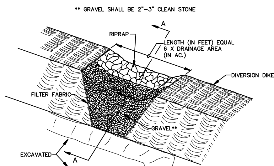
OUTLET (PERSPECTIVE) TEMPORARY SEDIMENT TRAP (ST) N.T.S.
