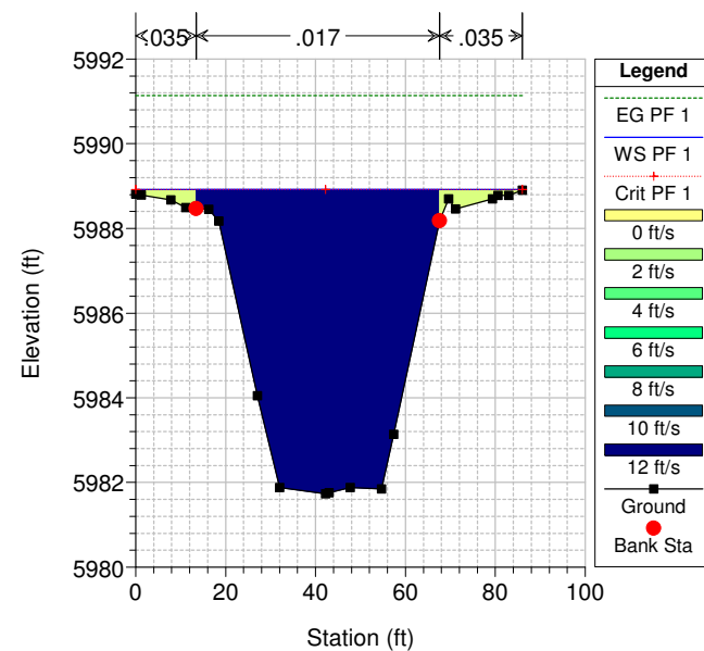
Geom: PINO ARROYO -EXST RS = 1251.03
