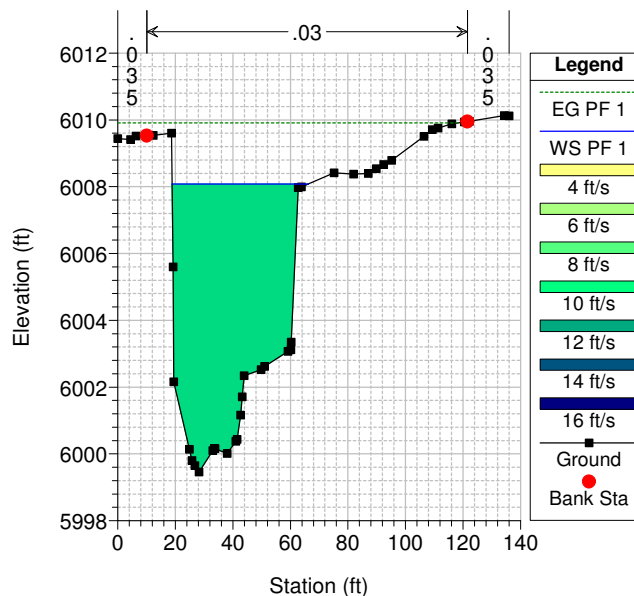
Geom: PINO ARROYO -EXST RS = 1807.37
