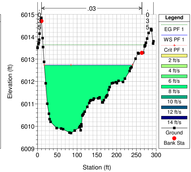
Geom: PINO ARROYO -EXST RS = 1891.58
