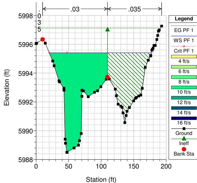
Geom: PINO ARROYO -EXST RS = 1426.03
