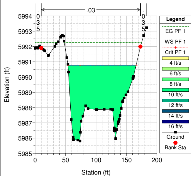
Geom: PINO ARROYO -EXST RS = 1350
