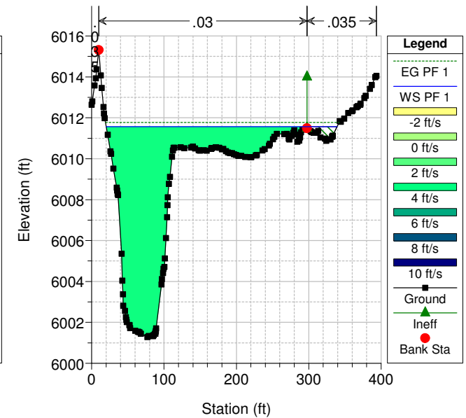
Geom: PINO ARROYO -EXST RS = 1873.47
