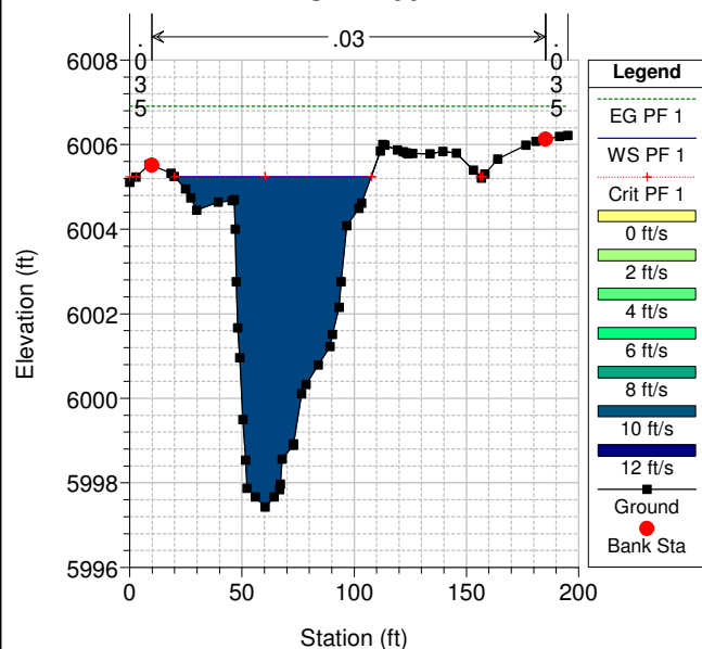
Geom: PINO ARROYO -EXST RS = 1700
