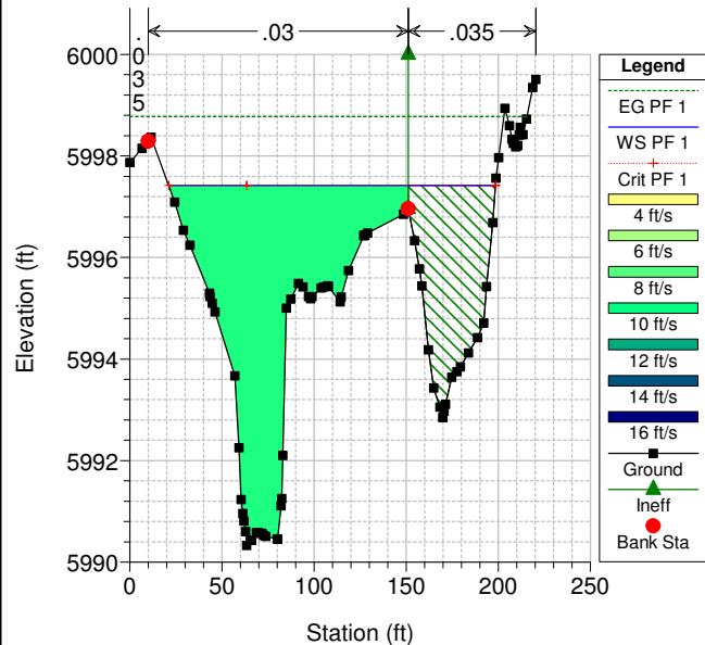
Geom: PINO ARROYO -EXST RS = 1481.63
