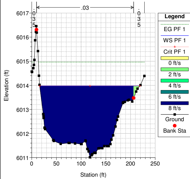
Geom: PINO ARROYO -EXST RS = 1901.89
