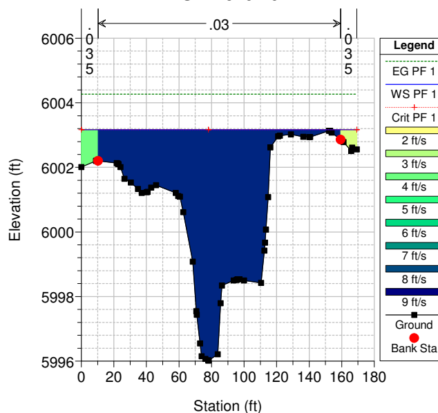
Geom: PINO ARROYO -EXST RS = 1629.49
