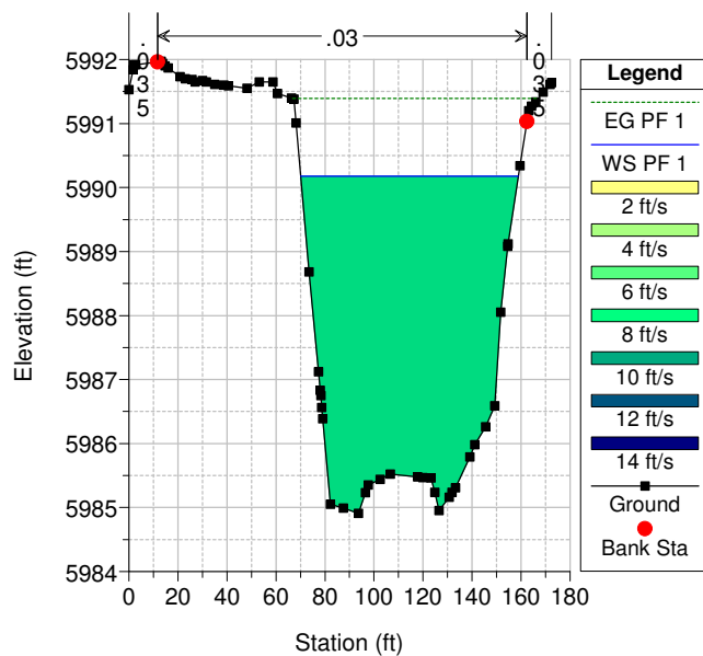
Geom: PINO ARROYO -EXST RS = 1310.72
