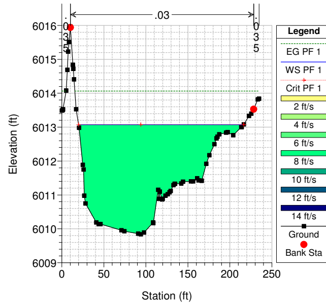
Geom: PINO ARROYO -EXST RS = 1898.1
