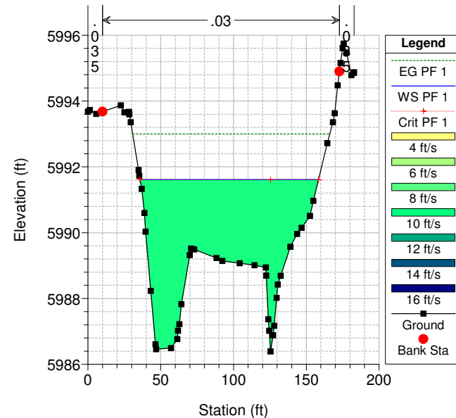
Geom: PINO ARROYO -EXST RS = 1370.42
