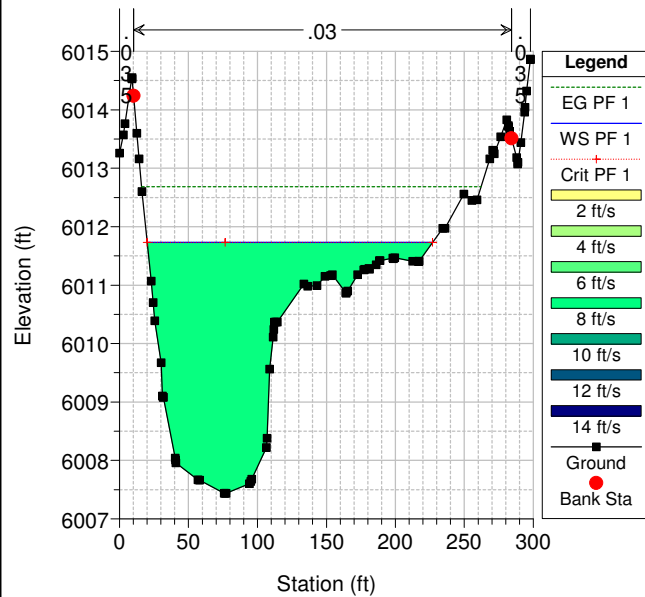
Geom: PINO ARROYO -EXST RS = 1887.76
