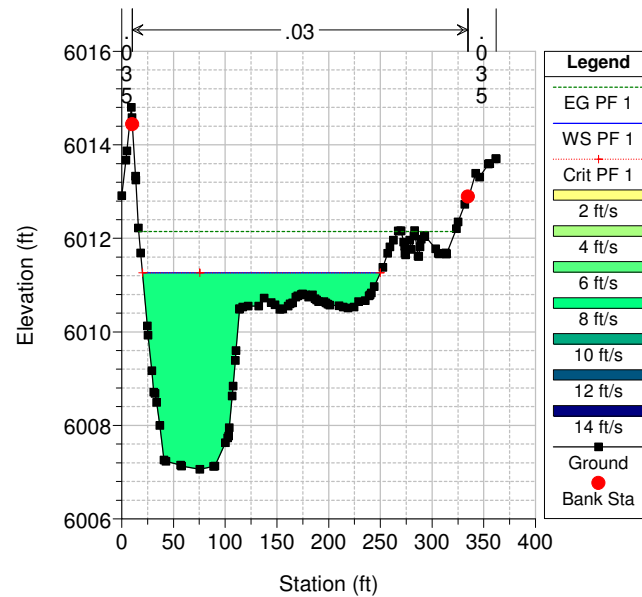
Geom: PINO ARROYO -EXST RS = 1878.66
