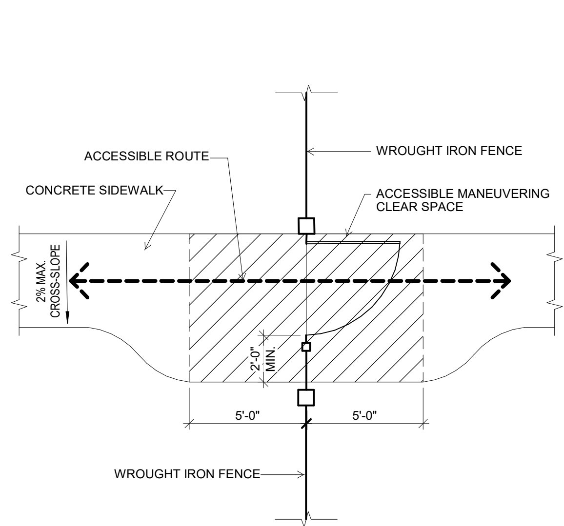
7 ACCESSIBLE MANEUVERING SPACE AT GATES SCALE: 1/4" = 1'-0"
