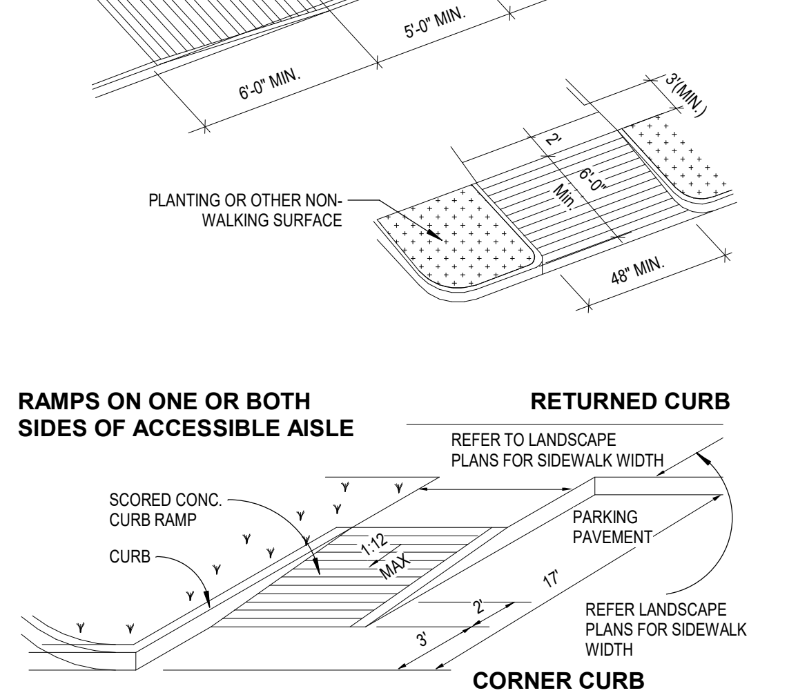
5 TYPICAL ACCESSIBLE RAMP SCALE: 1/4" = 1'-0"
