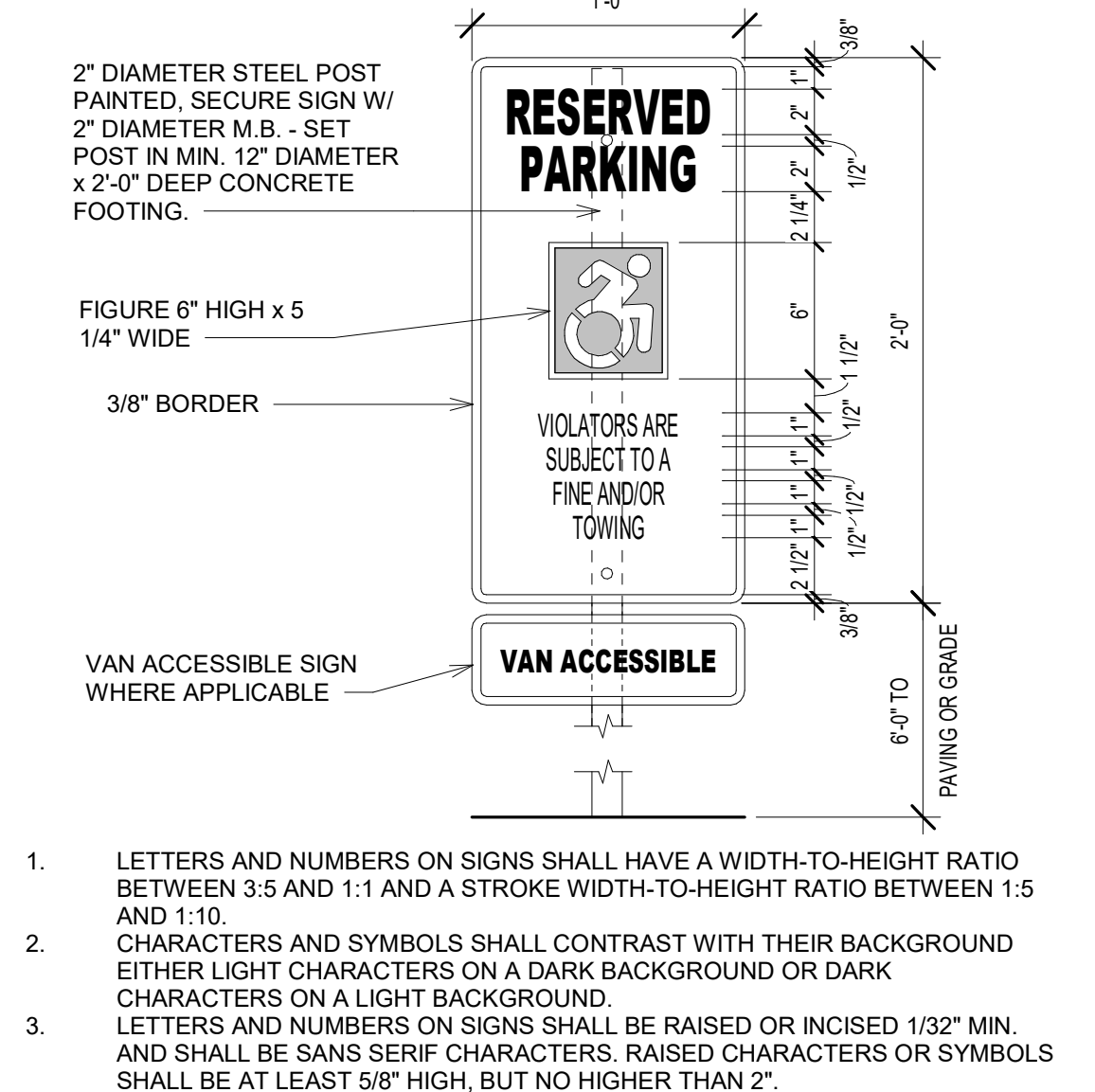
2 ACCESSIBLE PARKING SIGN SCALE: 1 1/2" = 1'-0"
