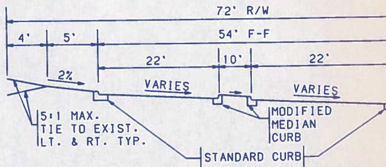
SUBDIVISION ENTRANCE STREET S
