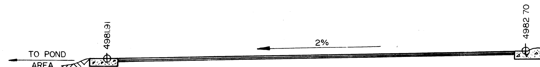
CROSS-SECTION AT 0+57 3/16" = 1'-0"
