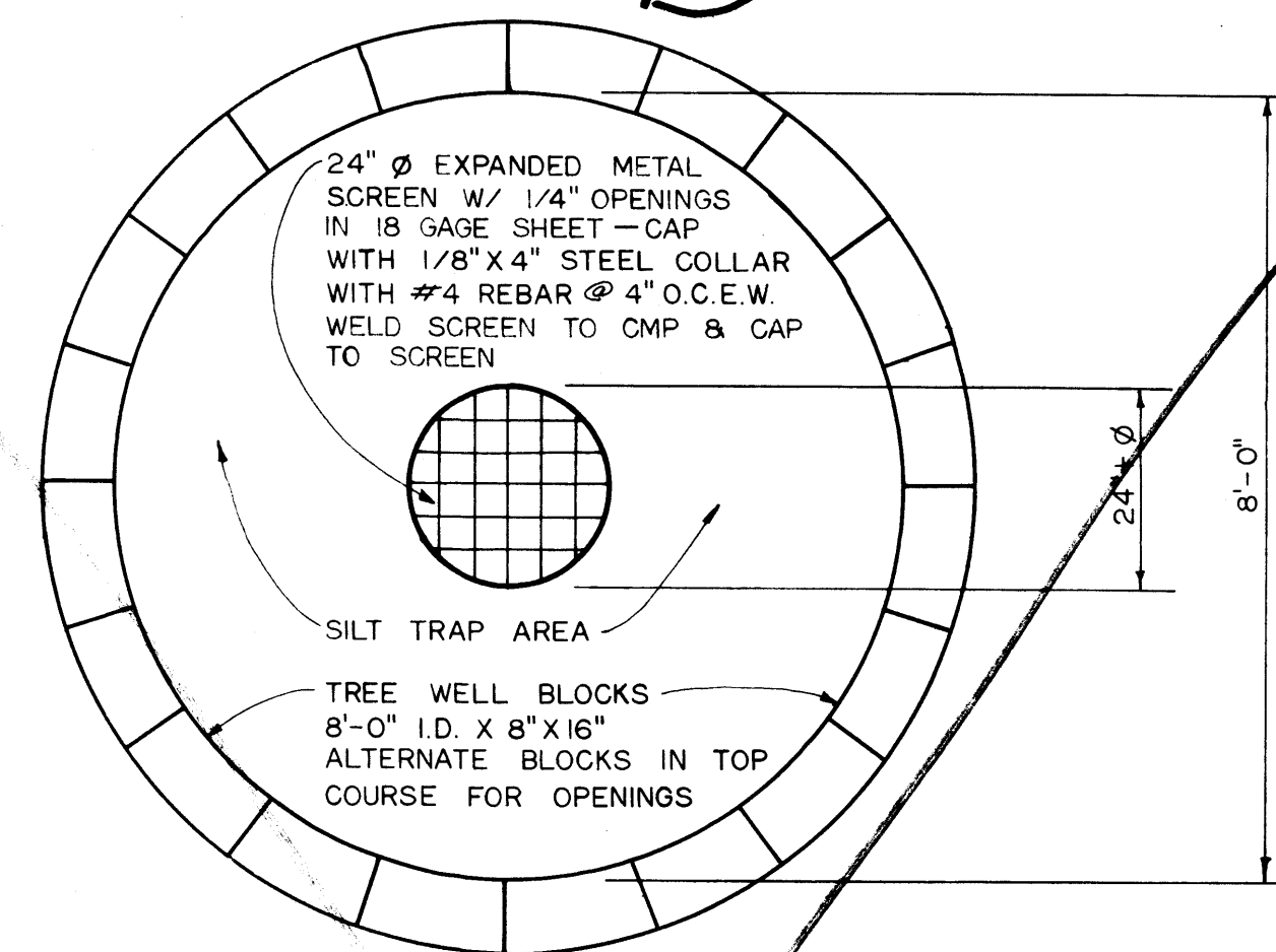
INJECTION WELL PLAN 1/2" = 1'-0" (SQUARE CONFIGURATION IS ACCEPTABLE)
