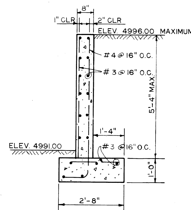
SUGGESTED RETAINING WALL (IF REQUIRED) 1/2" = 1'-0"
