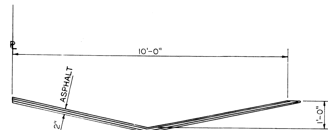
SWALE CROSS-SECTION AT NORTH R. OF SUBDIVISION AND WEST R. OF LOT 9 1/2" = 1'-0"
