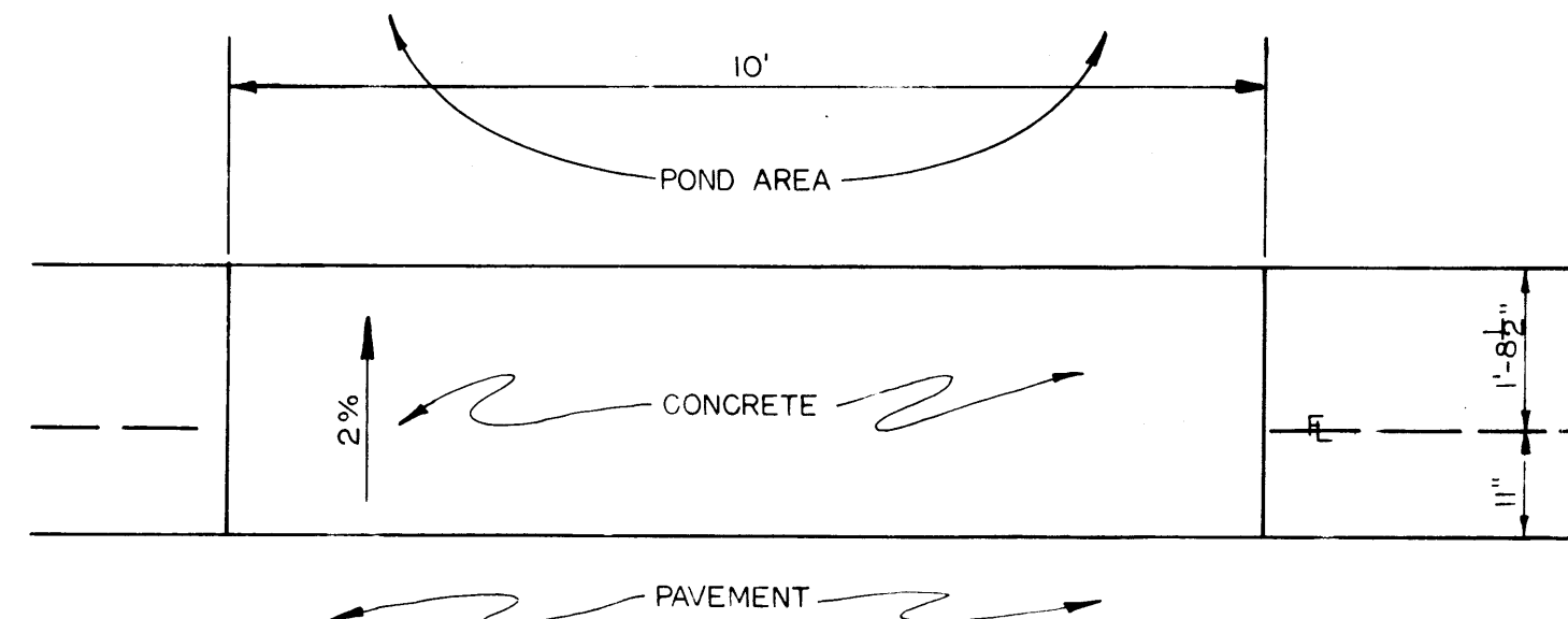
CURB RUNDOWN PLAN 1/2" = 1'-0"
