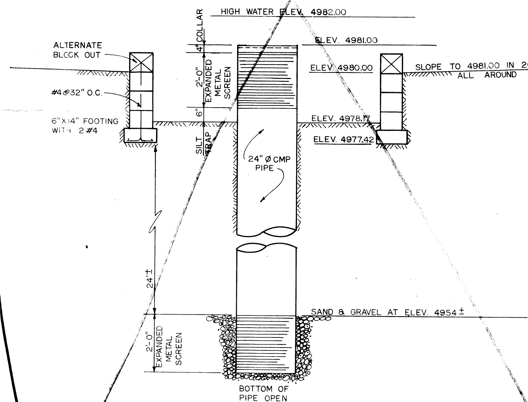
INJECTION WELL ELEVATION 1/2" = 1'-0"
