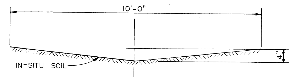
INDIVIDUAL LOT SWALES 1/2" = 1'-0"
