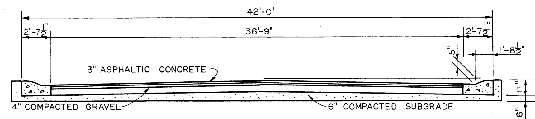
TYPICAL PAVEMENT SECTION 3/16" = 1'-0"
