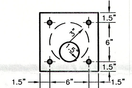
TYP. ORIFICE PLATE DETAIL NTS
