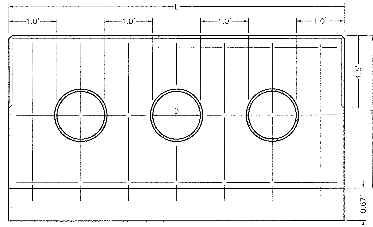
ELEVATION NTS
