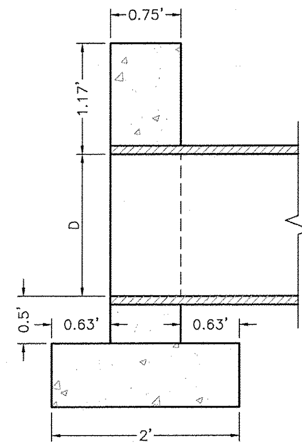
SECTION NTS
