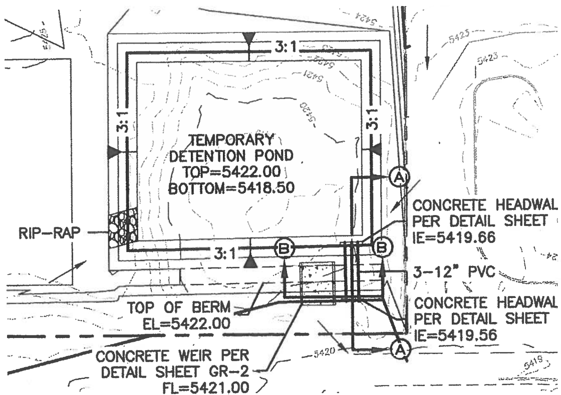
POND DETAIL
