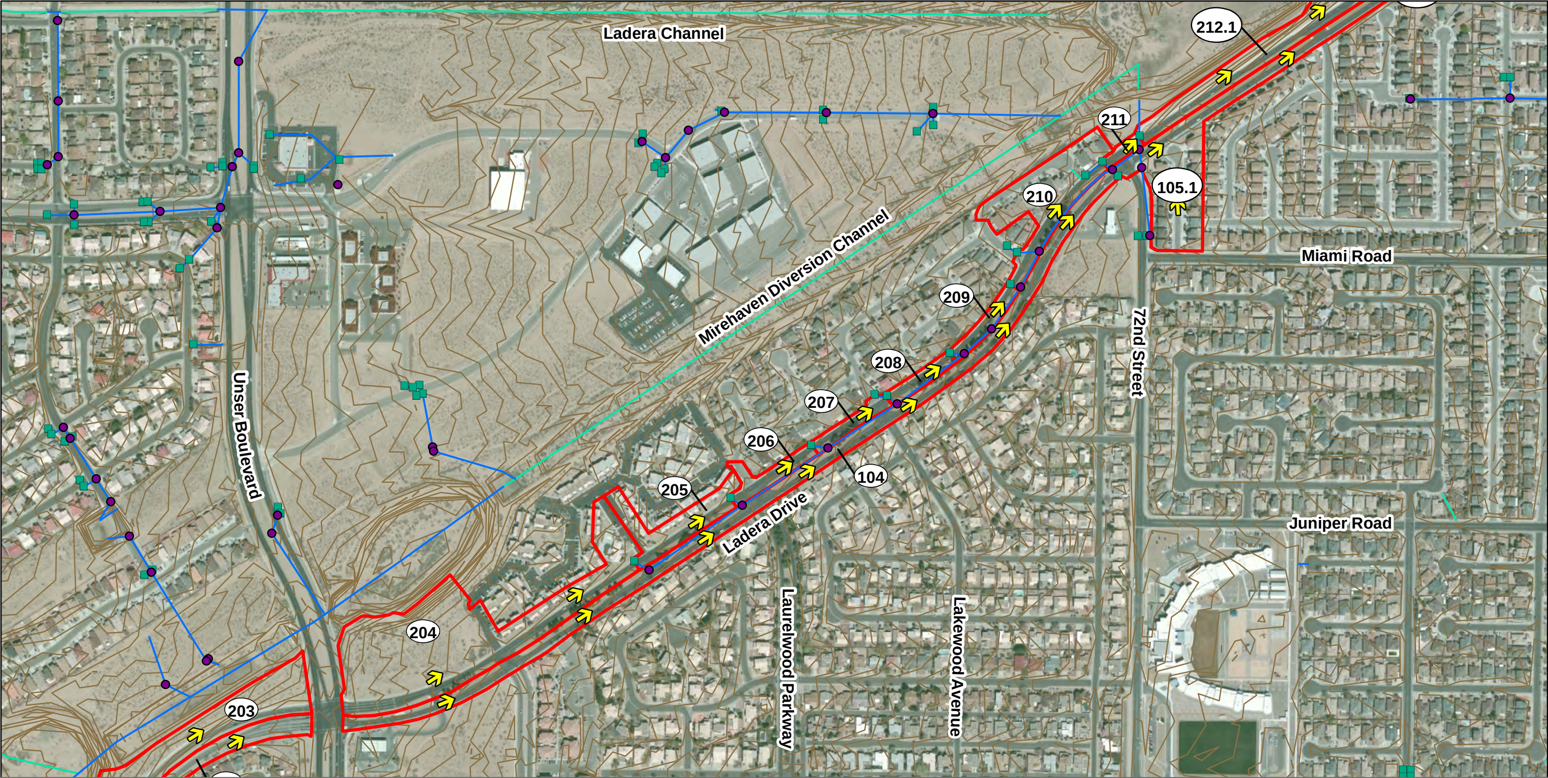
Exhibit 3 Drainage Basin Map (Unser Blvd. to 72nd St.) Ladera Drive Improvements
