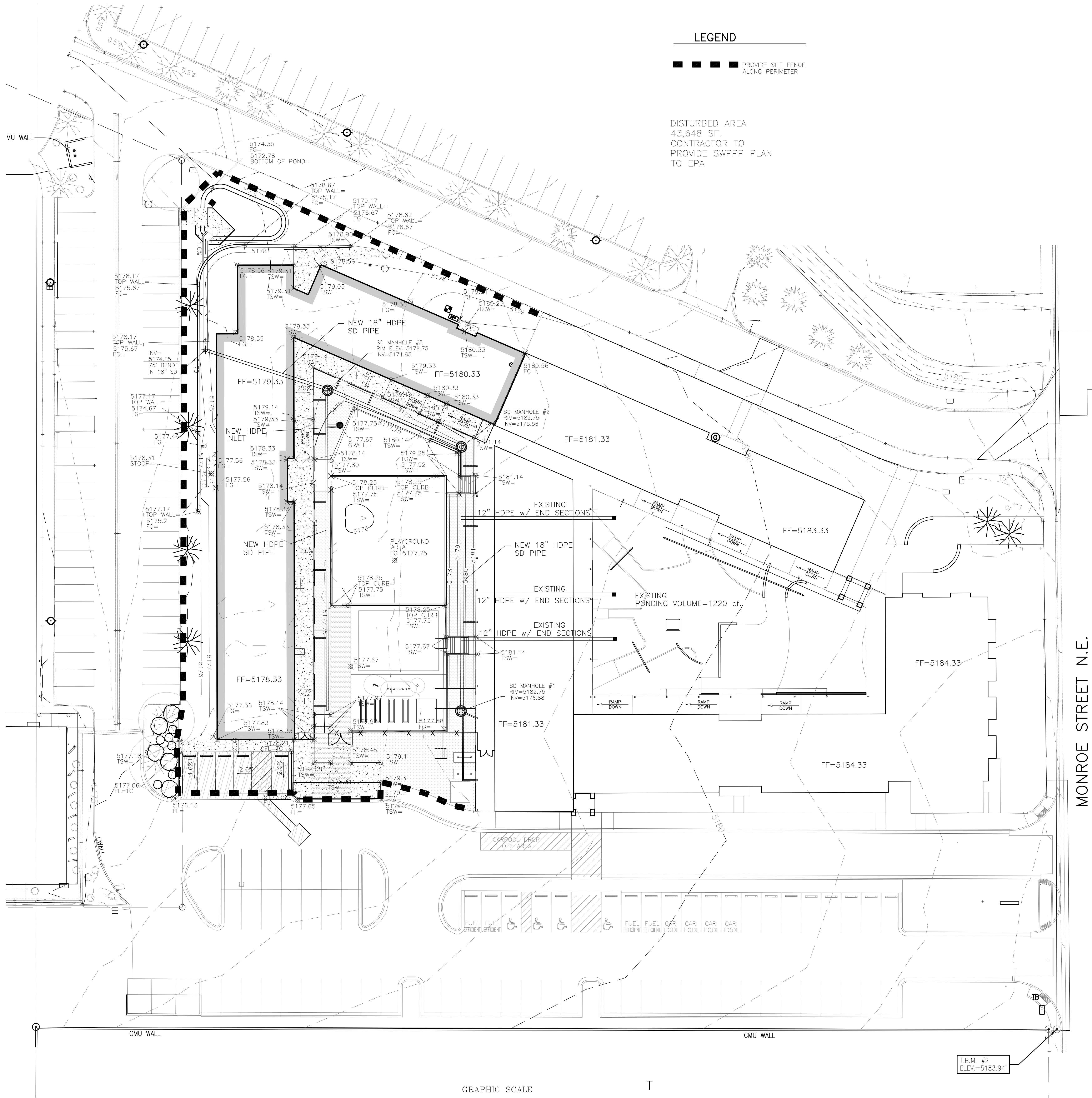
A1 EROSION AND SEDIEMTN CONTROL PLAN SCALE: 1" = 20'-0"
