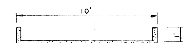
TYPICAL CROSS SECTION "B-B" (MIN. SLOPE 0.6 %)
