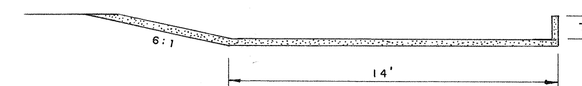
TYPICAL CROSS SECTION "A-A" (MIN. 0.5 % SLOPE)
