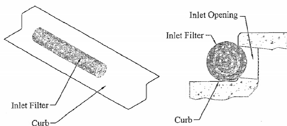
Cross-Section
