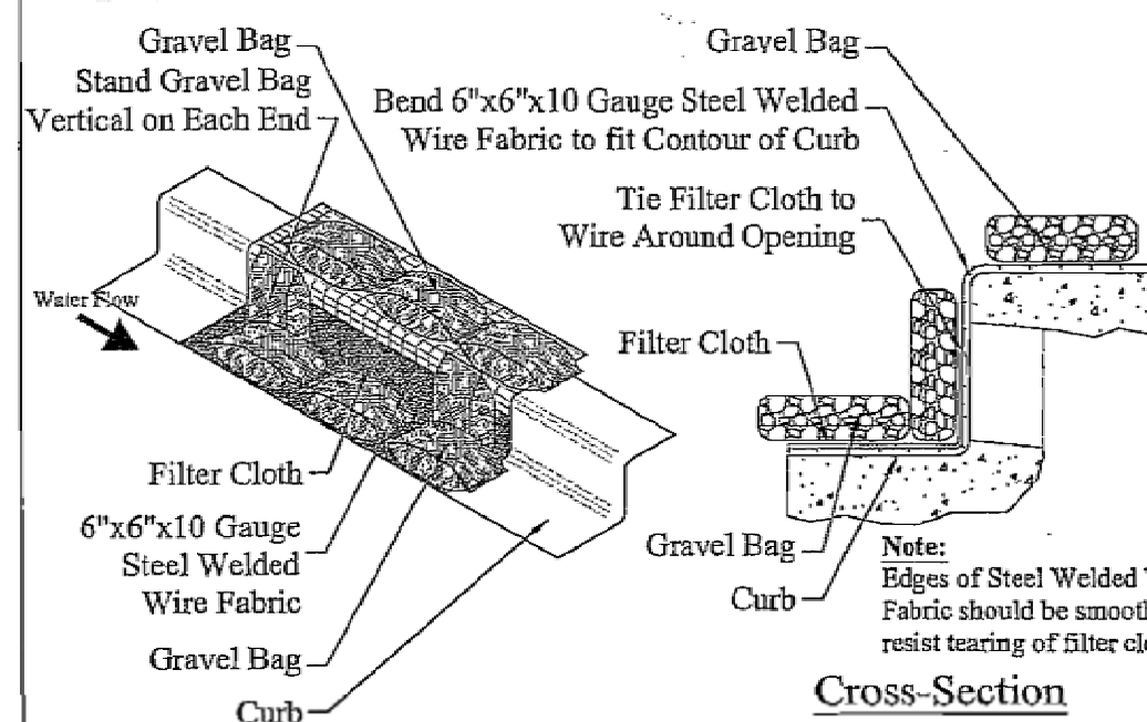
Cross-Section
